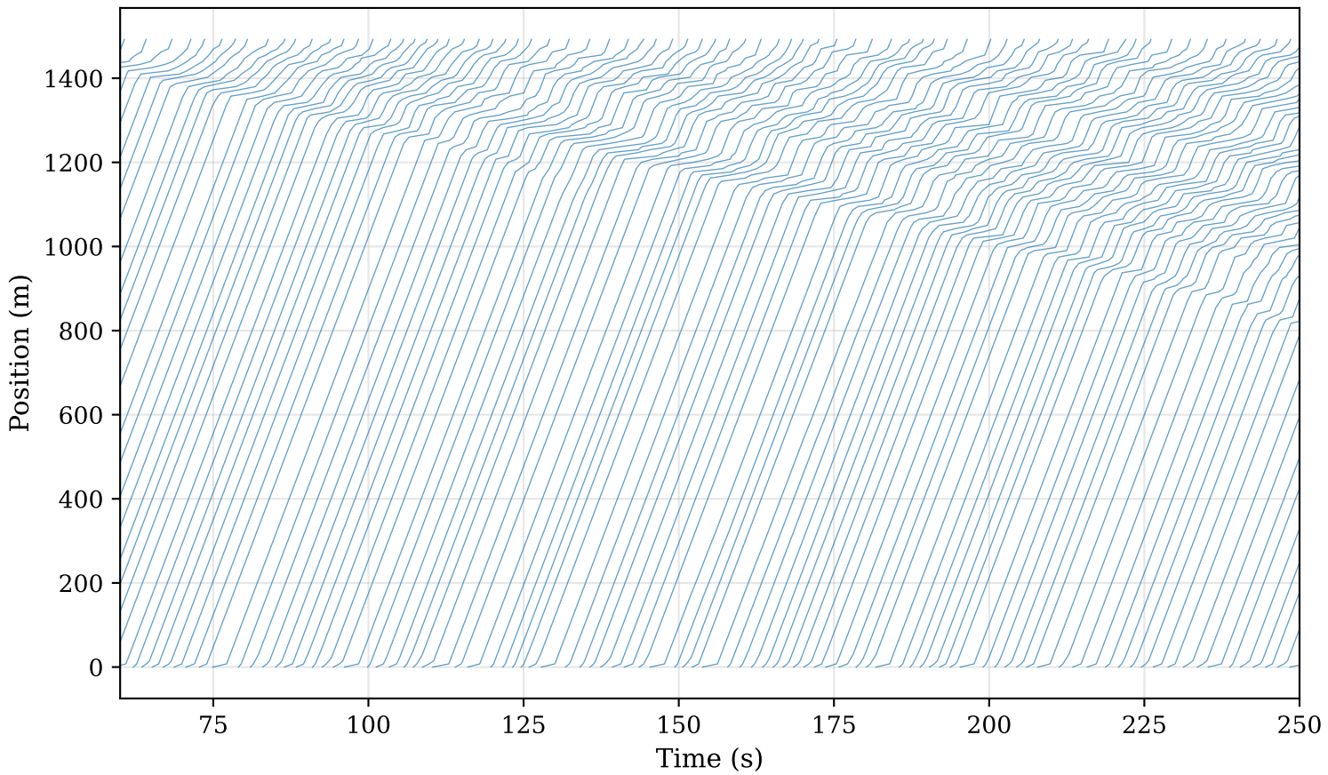
Time-Space Diagram: Congested
