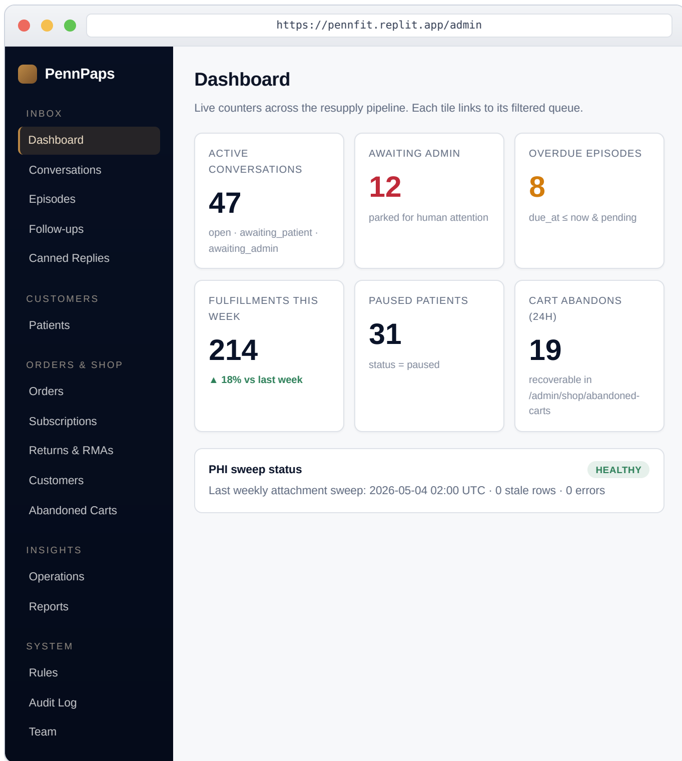
Figure 3 · The admin Dashboard. Click any KPI to land on its filtered queue.
