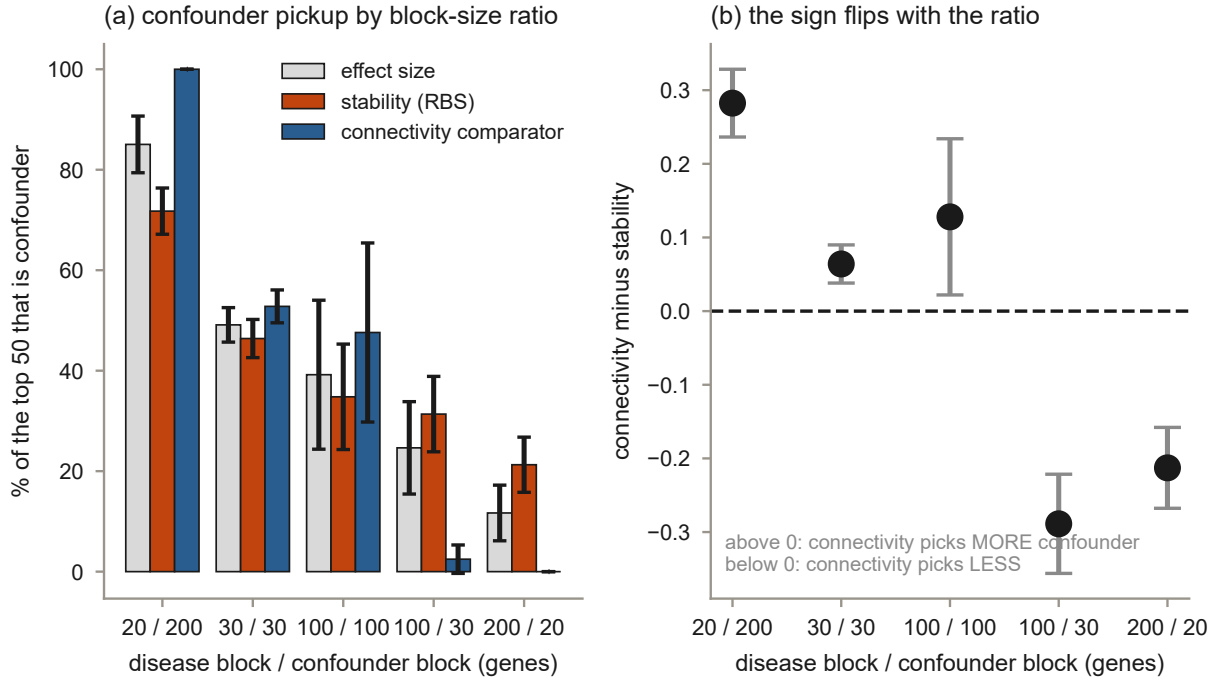
Figure S3: Connectivity criteria are biased by module size, which is why one method escaped. Simulation sweeping the ratio between the size of the disease block and that of the confounder block. a Percentage of the top 50 features that come from the confounder block. b The difference between a connectivity criterion and a stability criterion, which changes sign as the ratio crosses one. In the real data the immediate-early block contains 19 genes against 705 in the top-connectivity block, placing it in the regime where connectivity misses the confounder for reasons unrelated to robustness. All seven configurations are significant by Wilcoxon signed-rank on paired replicates.
