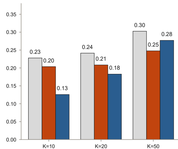
cross-fold Jaccard
