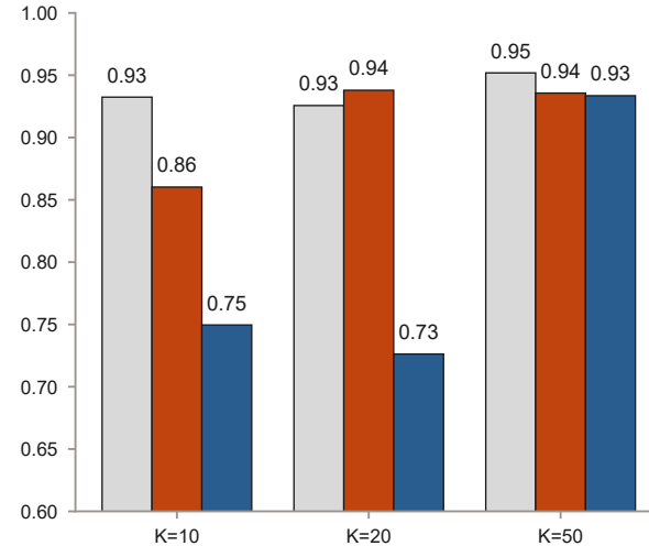
external AUROC
