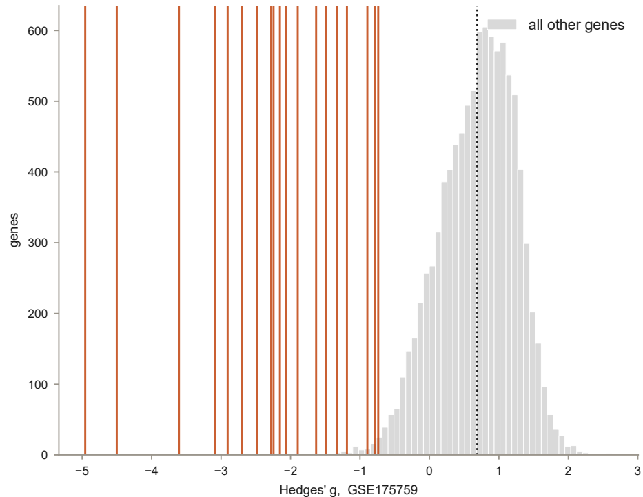
The module sits in the tail of the transcriptome Mann-Whitney p = 5.4e-14
