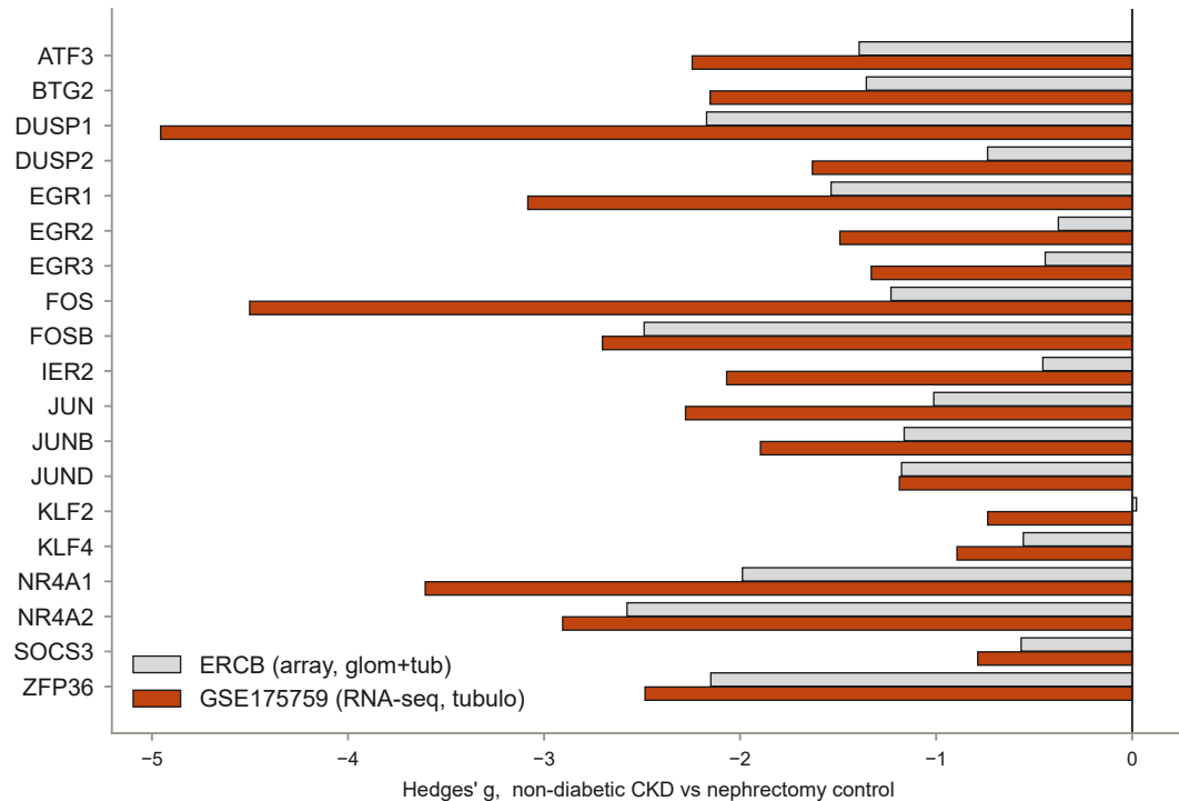
Immediate-early module, two independent cohorts
