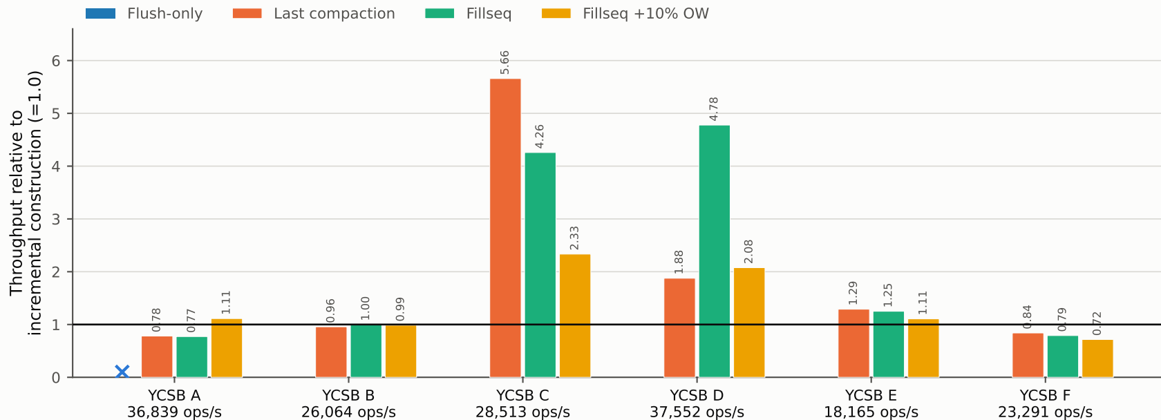
YCSB on each 1 TB loaded state: 300 s per cell, block cache 0, automatic compaction enabled
