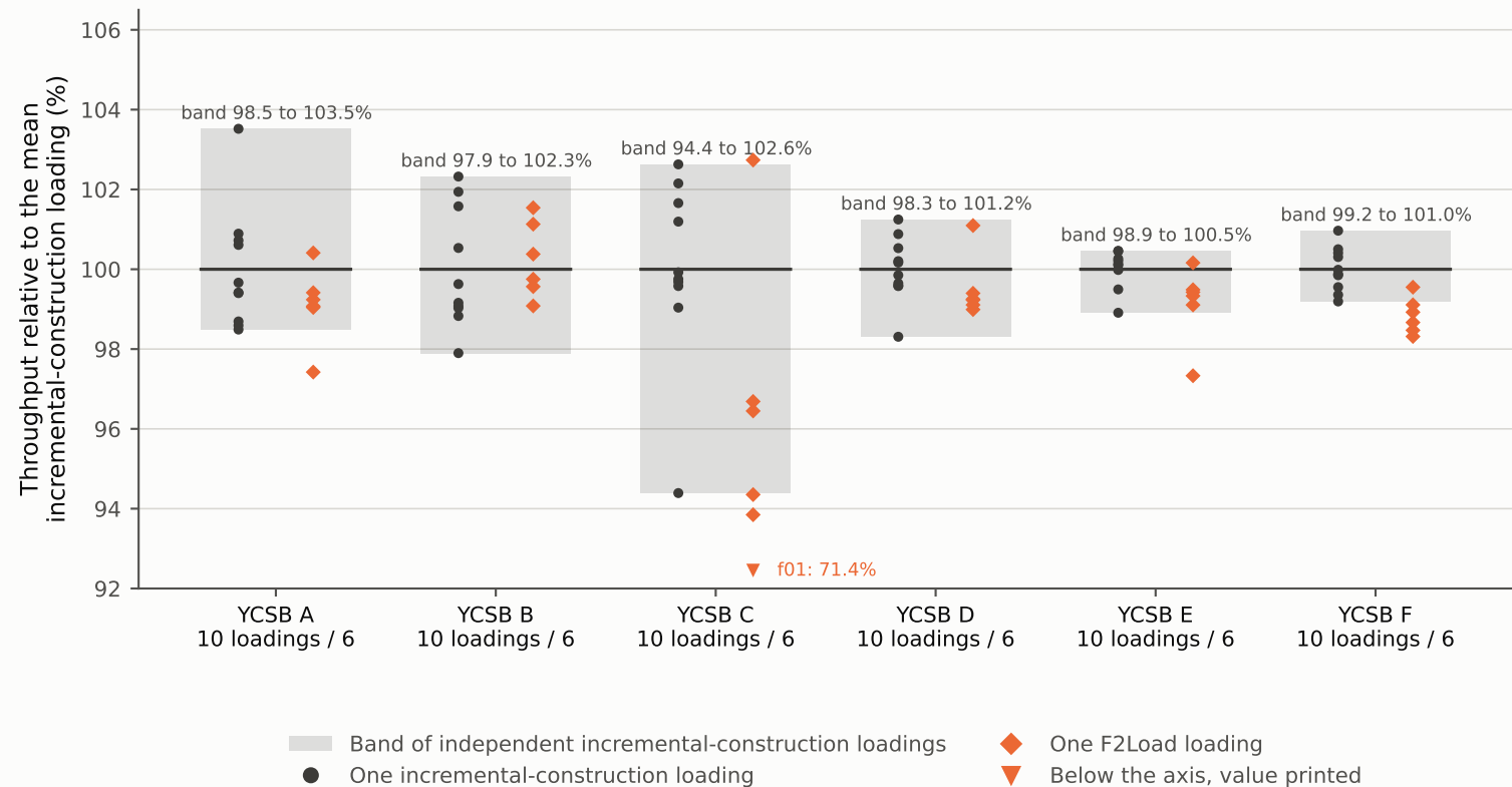
Run-to-run spread across independent 1 TB loadings: 300 s per cell, 50 GiB block cache
