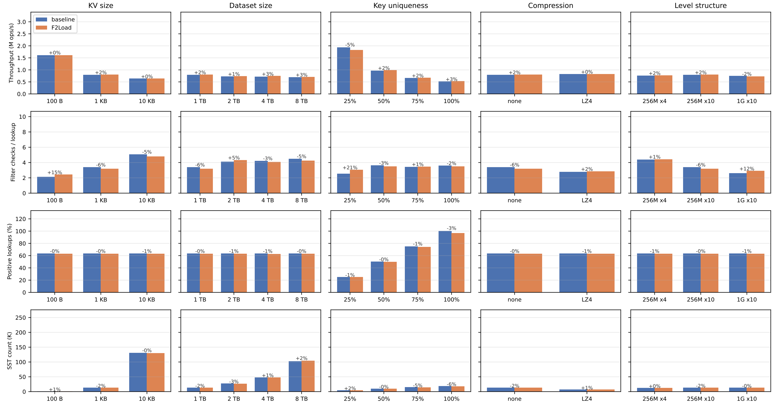
YCSB C (uniform, deep-copied DB; 48 threads, 300 s, 50 GiB cache): baseline vs F2Load, one option changed from P0 per group; labels = F2Load relative to baseline
