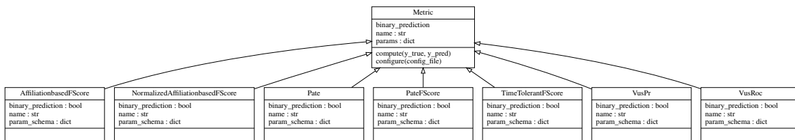
Figure 5.6: Temporal Shift-Tolerant Metrics class diagram
