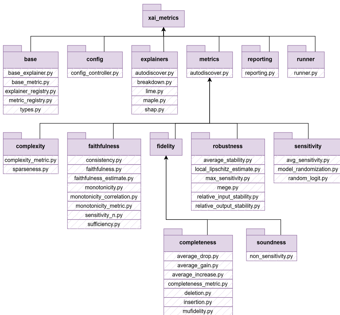
Figure 3.1: Architecture of XAIMetrics library
