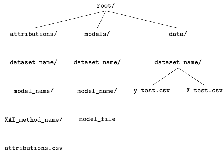
Figure 3.3: Directory structure used by XAIMetrics.
