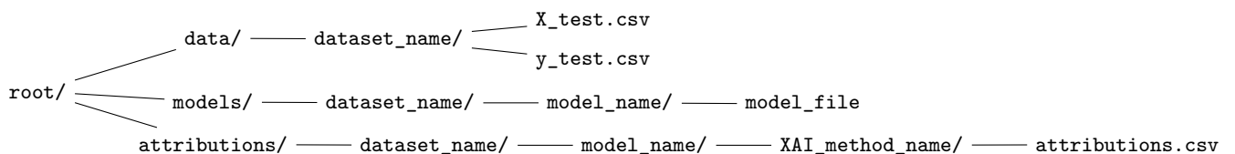
Figure 3.2: Directory structure used by XAIMetrics.
