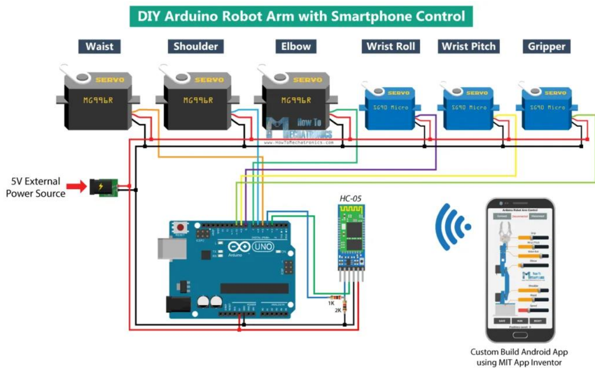
Circuit diagram
