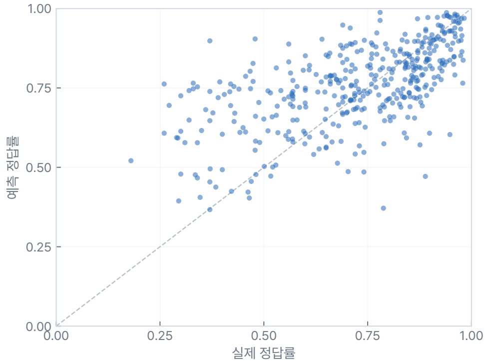
Predictor-1.0
