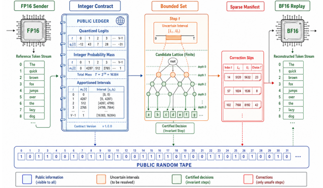
Figure 1: System architecture. The public integer contract converts a precision-sensitive distribution into a finite object. BDS stores only steps whose reachable decision set is not the reference singleton. This non-data illustration is generated from the prompt recorded in IMAGEGEN_PROMPTS.md.
