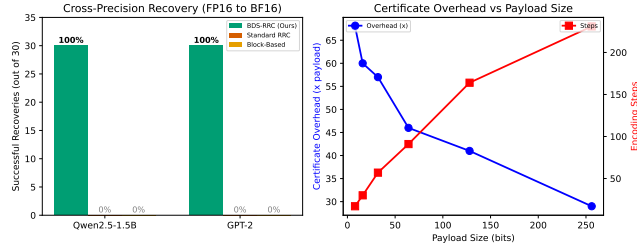
Figure 9: Main results. Left: BDS-RRC achieves 100% recovery; baselines 0%. Right: overhead decreases with payload size.
