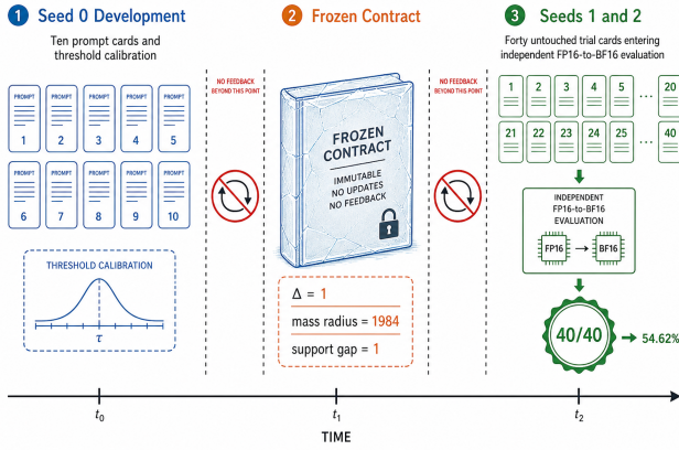
Figure 4: Frozen evaluation protocol. Seed 0 was used for mechanism development. Thresholds and implementation were then frozen before evaluating seeds 1 and 2.
