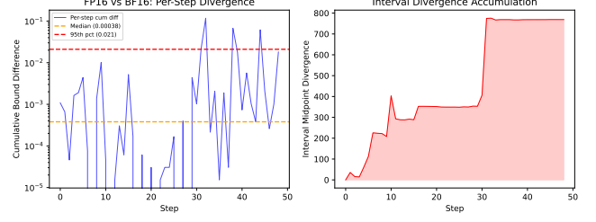
Figure 8: Error accumulation across precisions. Left: per-step cumulative bound difference. Right: interval midpoint divergence. Small per-step differences compound to large final errors.
