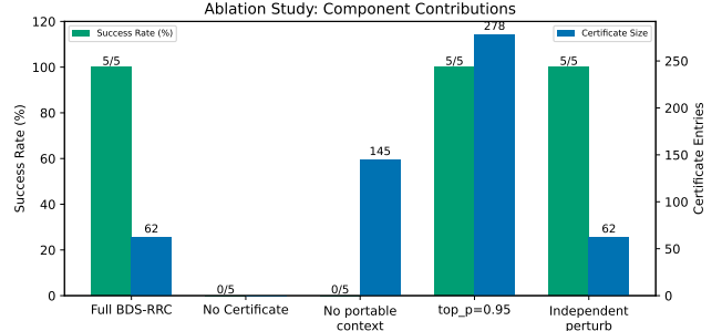
Figure 10: Ablation results. The correction certificate and portable precision context are necessary (0% without them).
