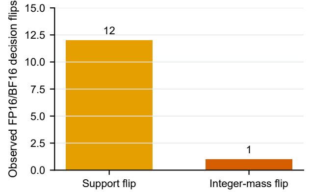
Figure 2: Observed failure anatomy in the frozen R056 development bundle. Support changes dominate but do not eliminate same-support mass changes, motivating joint enumeration.
