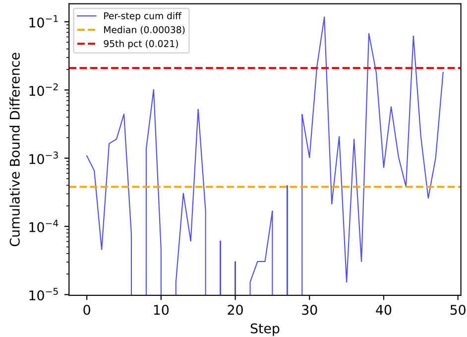
FP16 vs BF16: Per-Step Divergence
