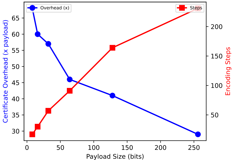
Certificate Overhead vs Payload Size
