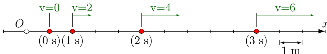
Figure 2: The position and velocity of a particle at times t = 0, 1, 2, 3 s if its motion is given as x(t) = 1 + t^2 and v(t) = 2t .
