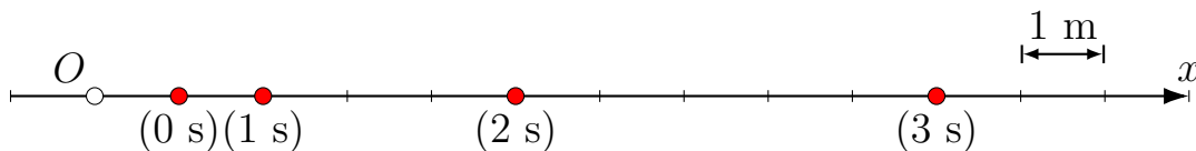
Figure 1: The position of a particle at times t = 0, 1, 2, 3 s if its motion is given as x(t) = 1 + t^2 .
