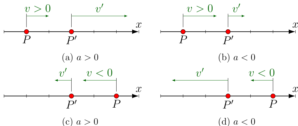
Figure 3: A particle is initially at P with the velocity as shown. A small time interval later, the particle is at location P' with a new velocity. For each of the four cases, determine if the acceleration is positive or negative.
