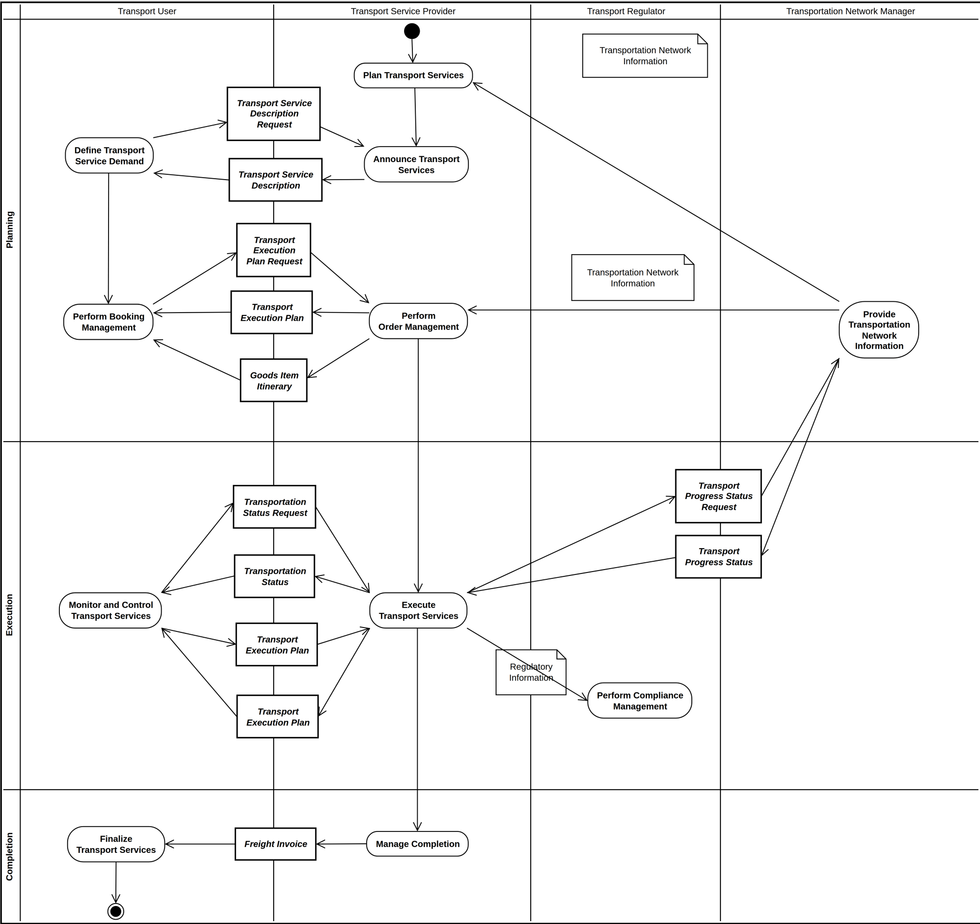
UBL-2.2-IMFM-IntermodalFreightManagementProcess: 275 × 258 mm; needs an A3 page.
