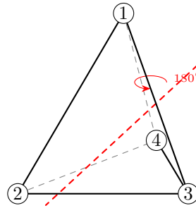
Rotation (13)(24)
