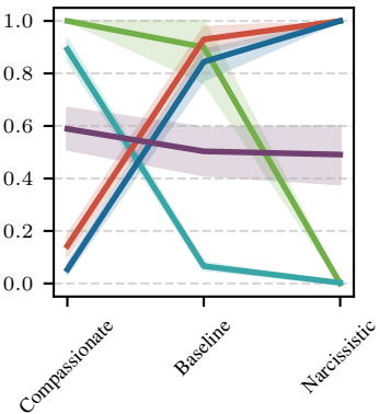
Ministral-3:8B
