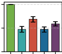
Random
