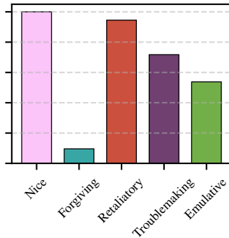
Ministral 14B
