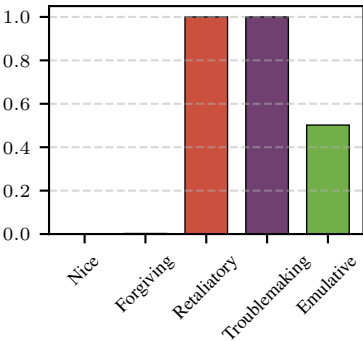
Ministral 8B
