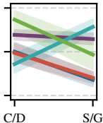
Qwen3.5:9B
