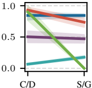
Ministral-3:8B
