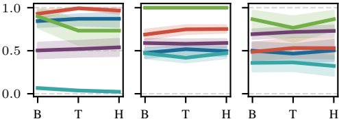
Qwen3.5:9B
