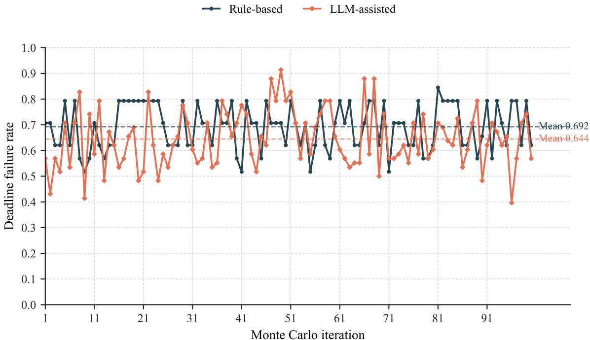
Deadline Failure Rate Across 100 Paired Monte Carlo Iterations
