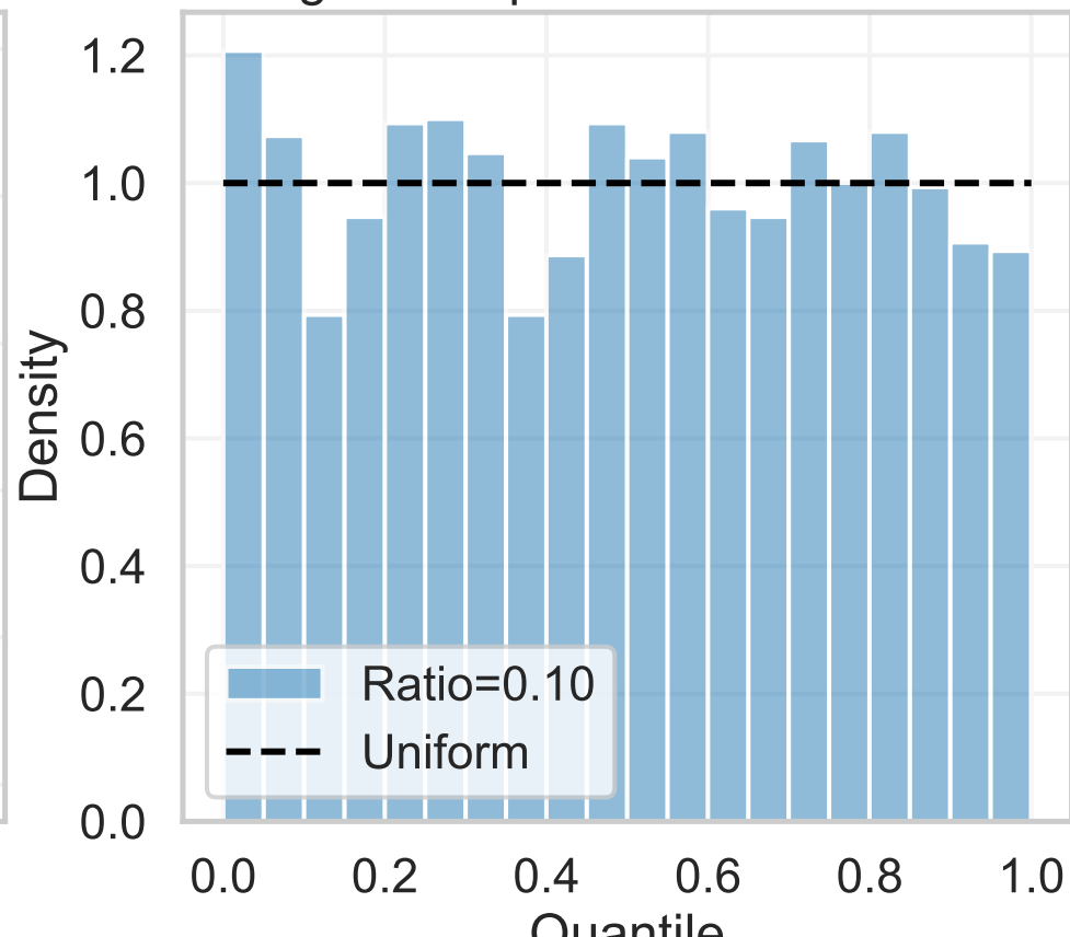
Histogram of quantiles over 3000 trials
