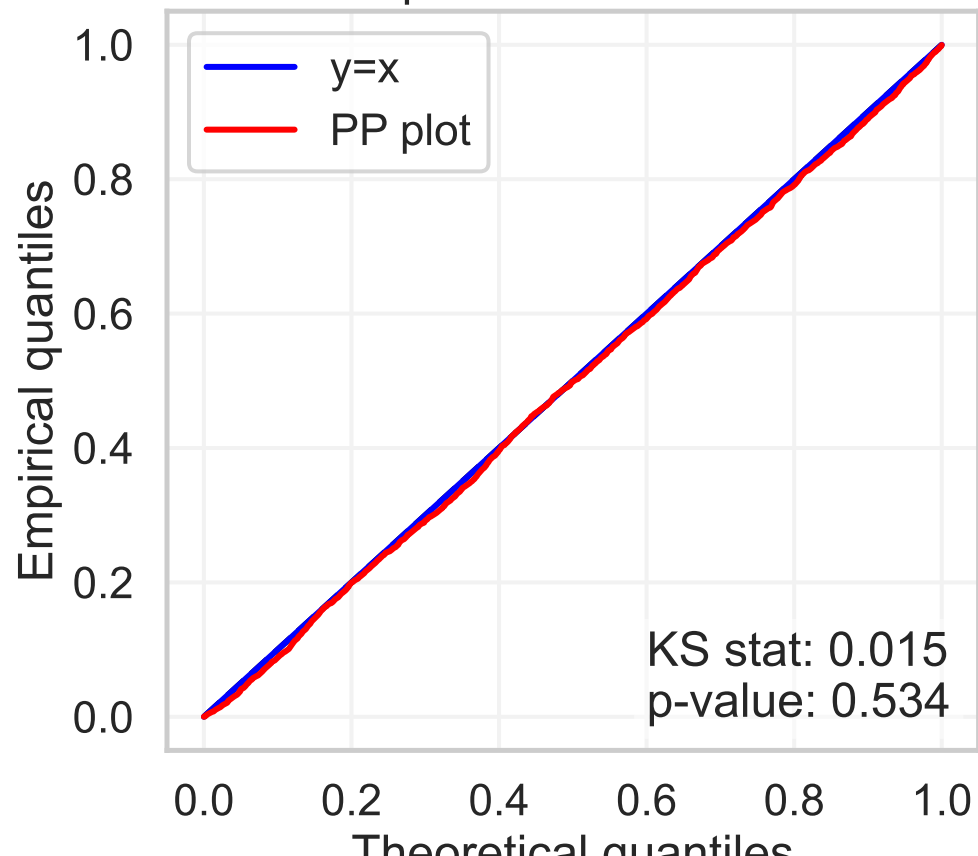
PP plot over 3000 trials
