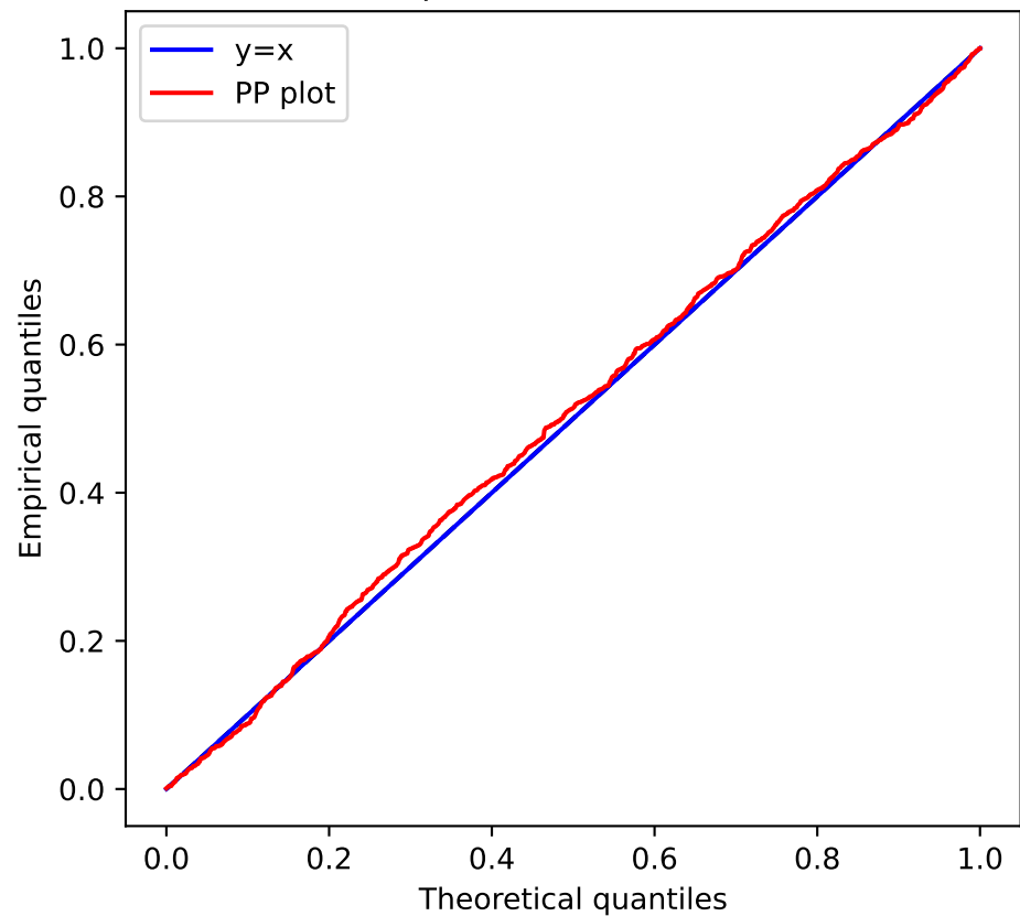
PP plot over 1000 trials
