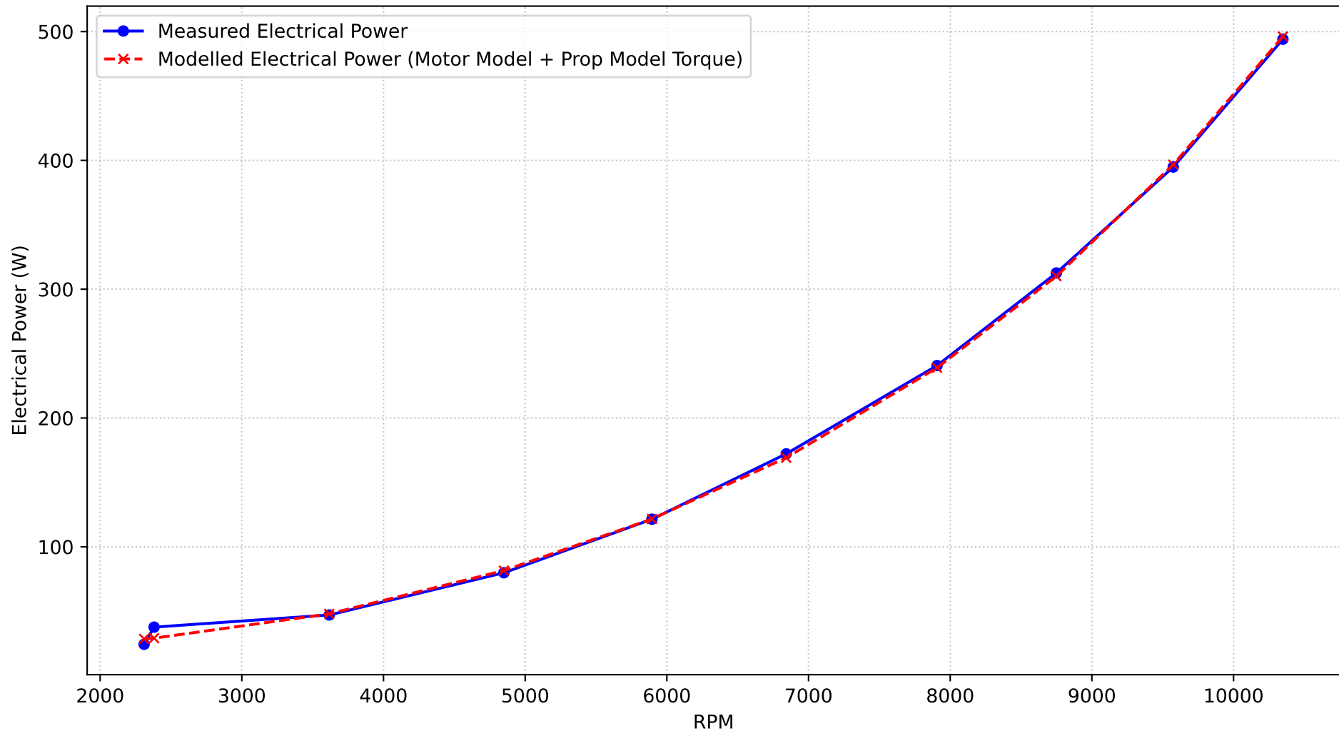
Measured vs Modelled Electrical Power for throttle_Speed_th1200.csv (Motor Model + Propeller Cq=2.454e-07)
