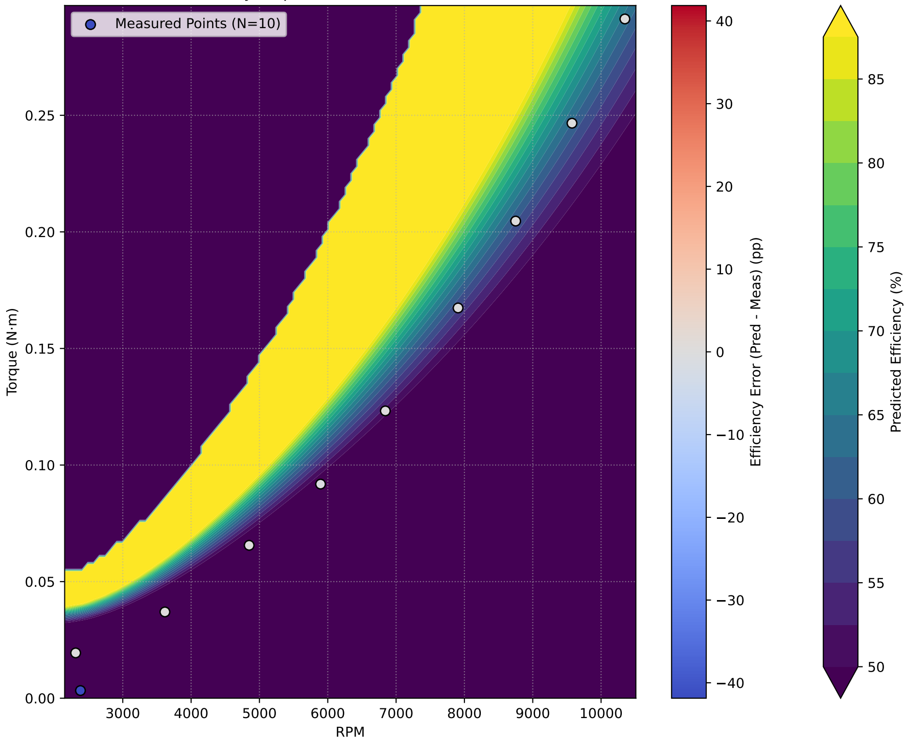
Motor Efficiency Map (Derived from Power Fit) - All Data
