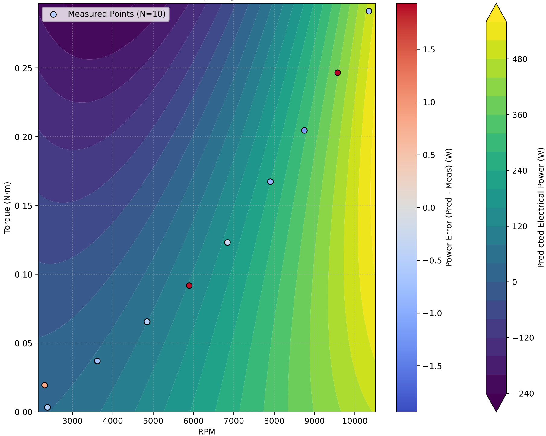
Motor Electrical Power Map (Polynomial Fit) - All Data
