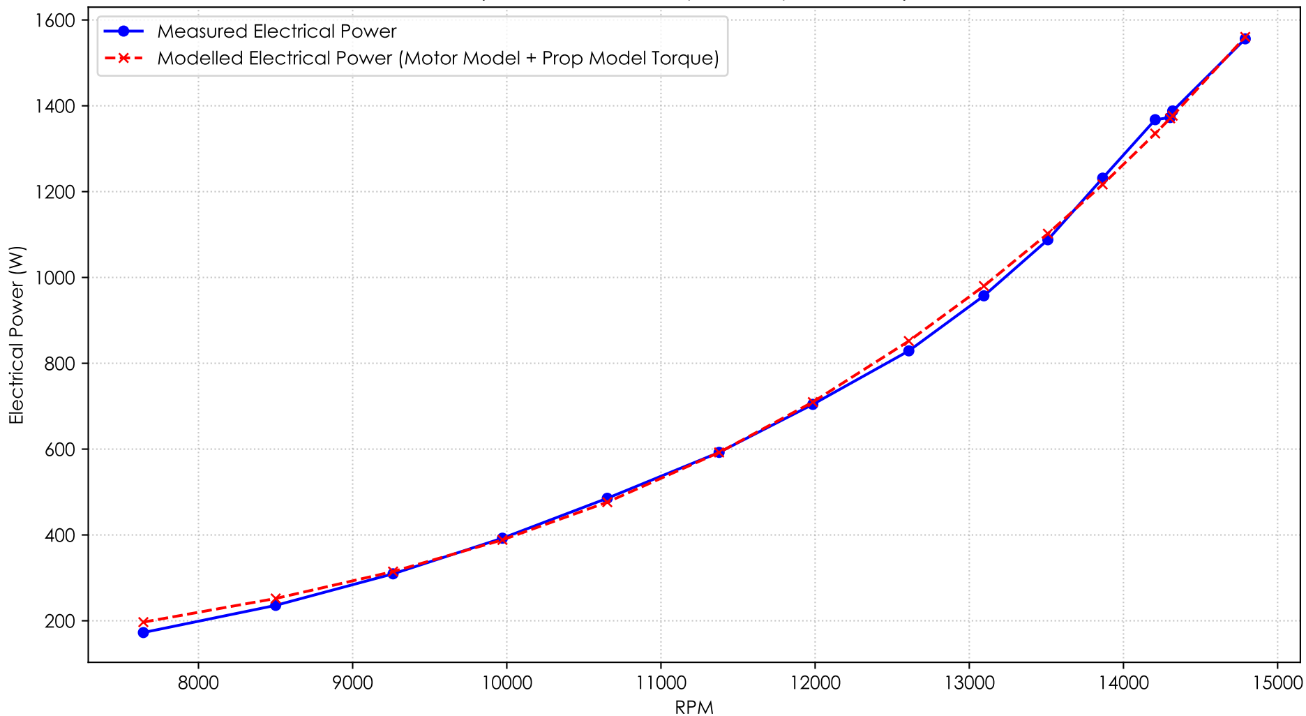
Measured vs Modelled Electrical Power for ARC_P43_10002199_32187_correlation_steps_01_manual.csv (Motor Model + Propeller C q =2.703e-07)
