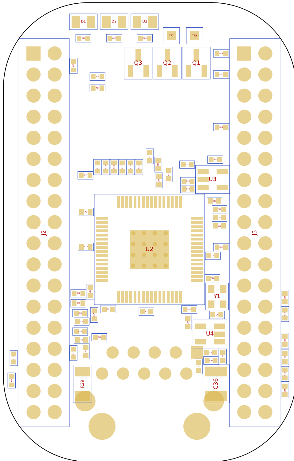
pocketbeagle2_ethernet_cap rev B - assembly TOP (all assembled SMD parts, J2/J3)
