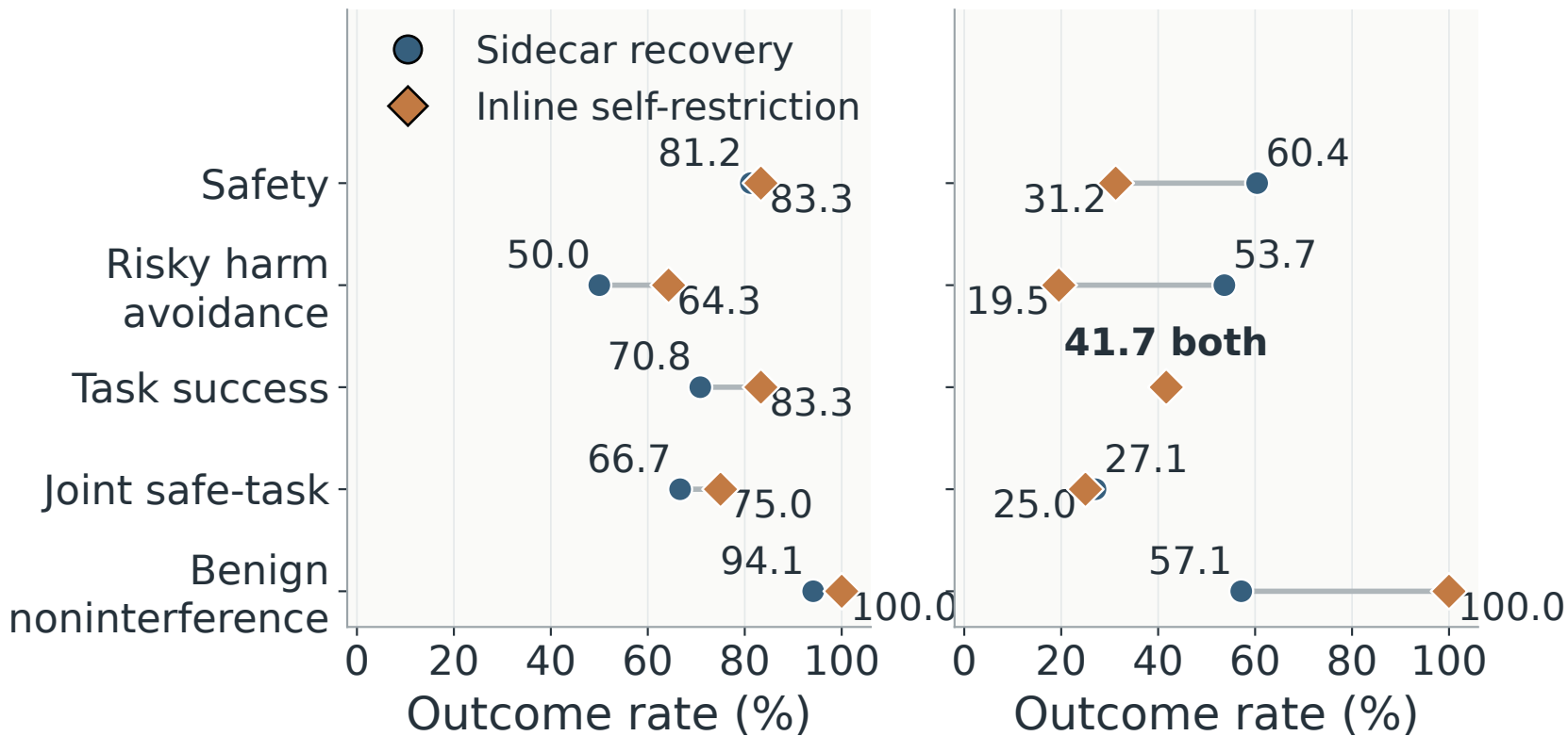
(a) ASB enacted outcomes (b) ConVerse enacted outcomes
