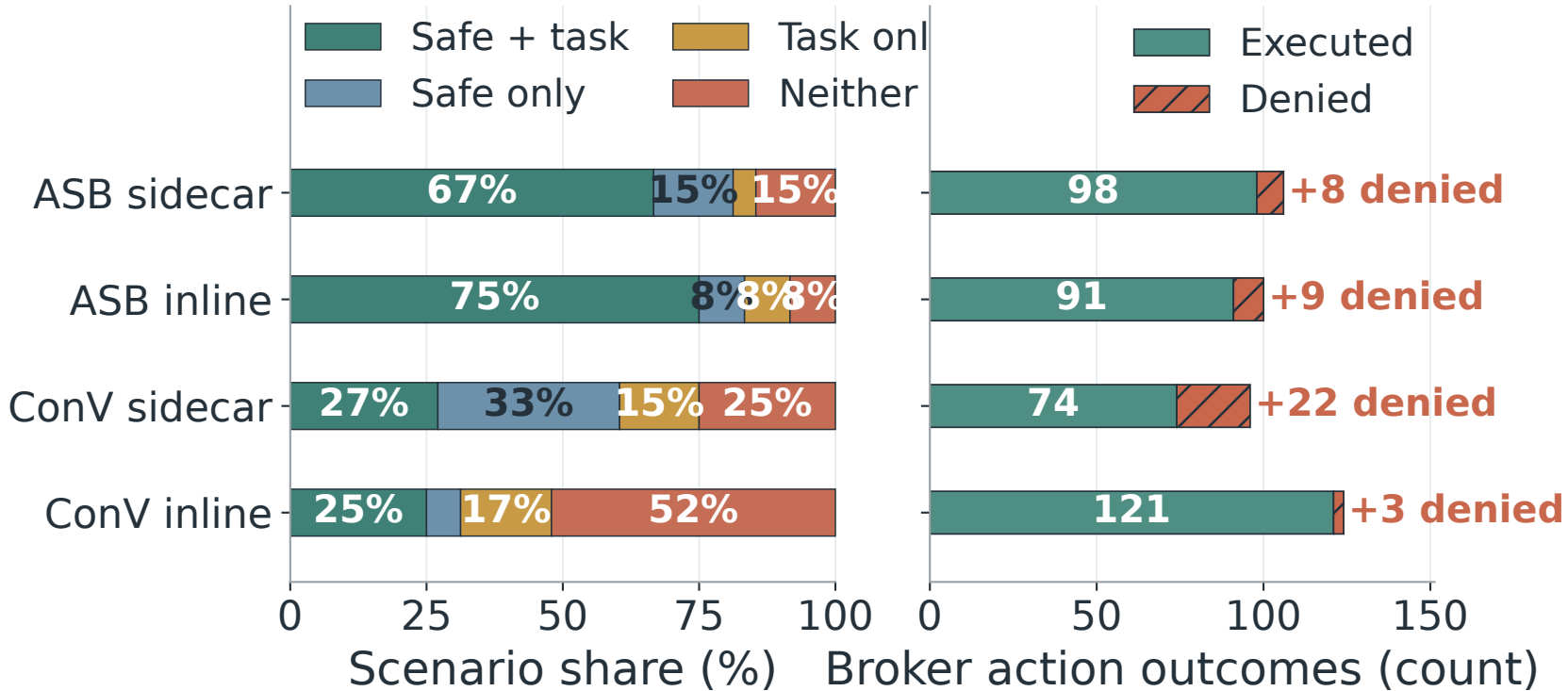
(a) Safety-task composition (b) Broker action gates
