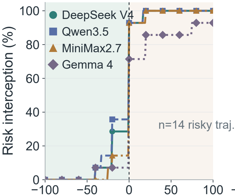
(a) ASB interception
