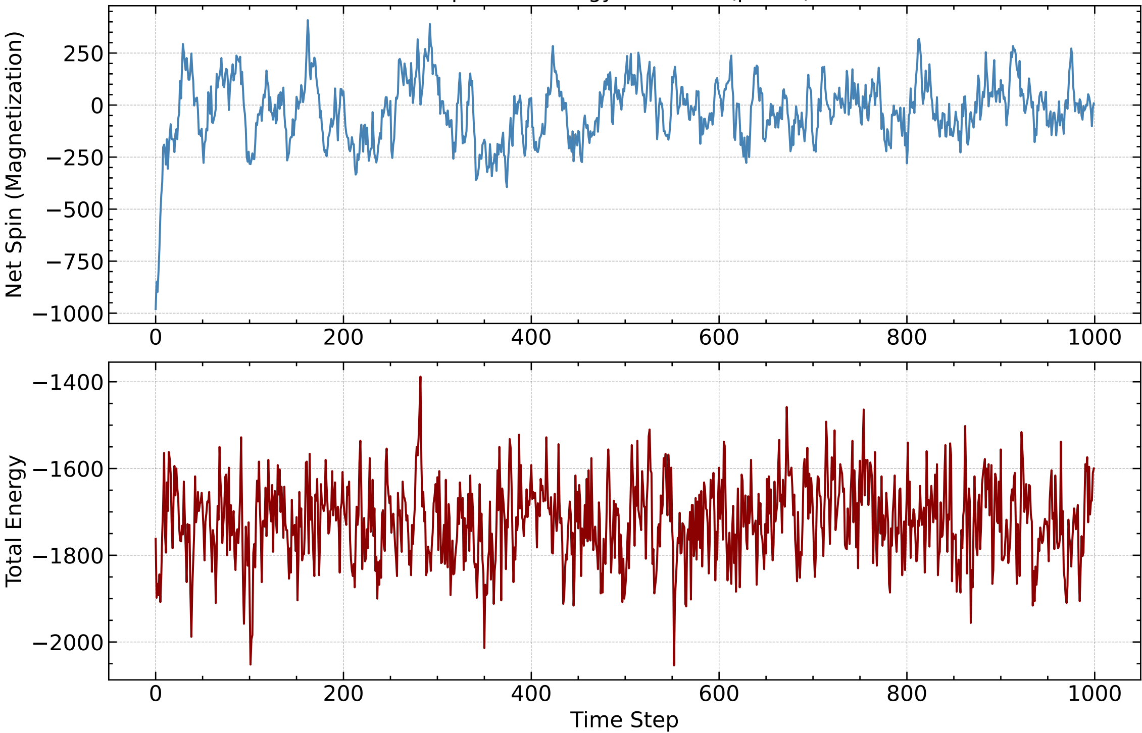
Spin and Energy Evolution ( \beta=0.3 )
