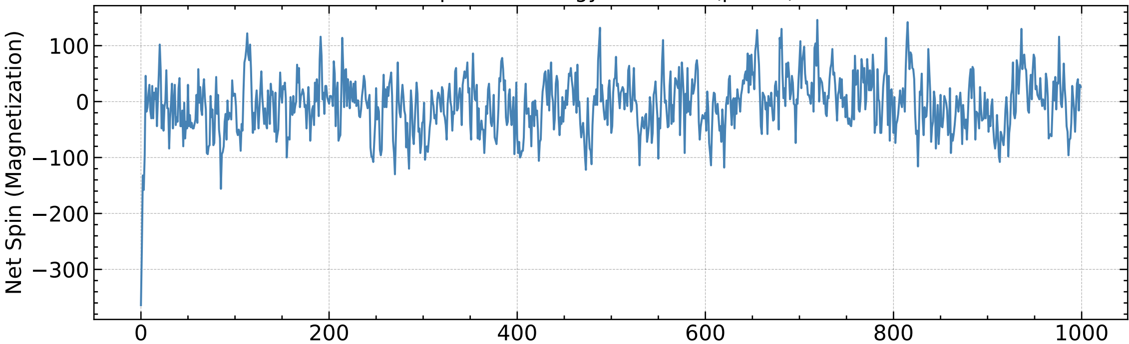
Spin and Energy Evolution ( \beta=0.2 )
