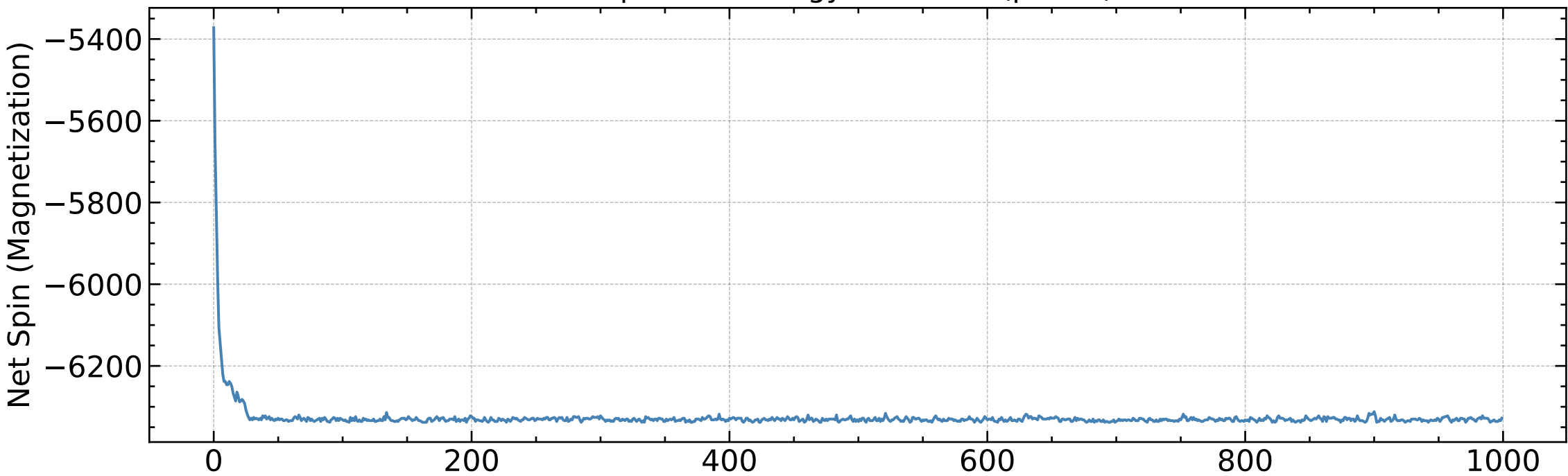
Spin and Energy Evolution ( \beta=0.9 )
