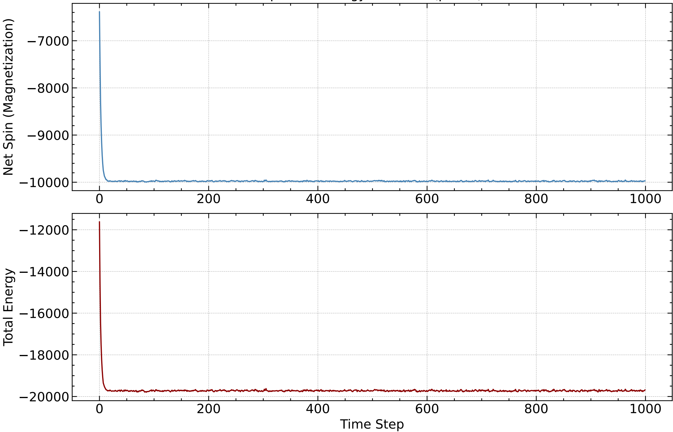
Spin and Energy Evolution ( \beta=0.9 )
