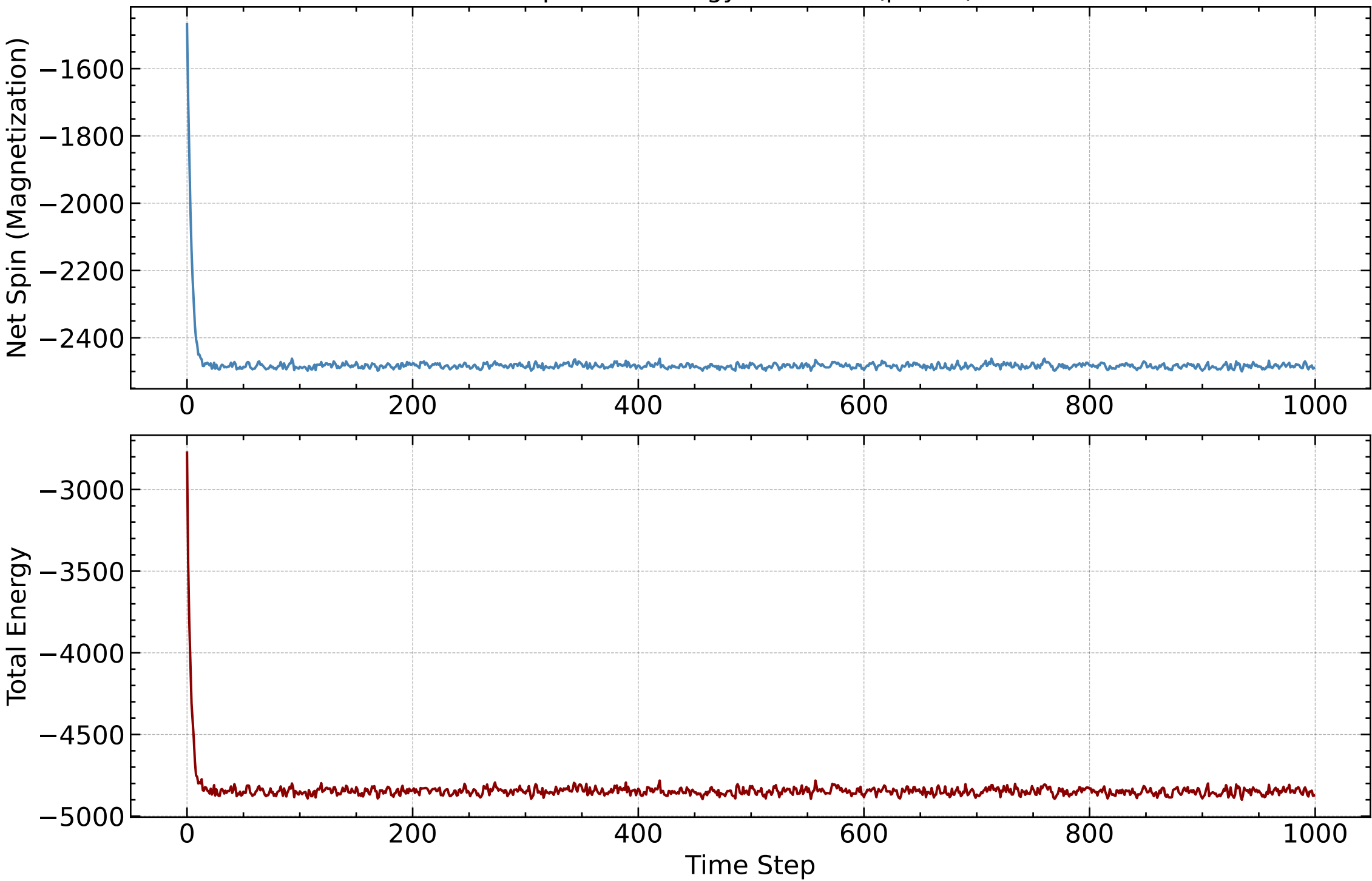
Spin and Energy Evolution ( \beta=0.8 )
