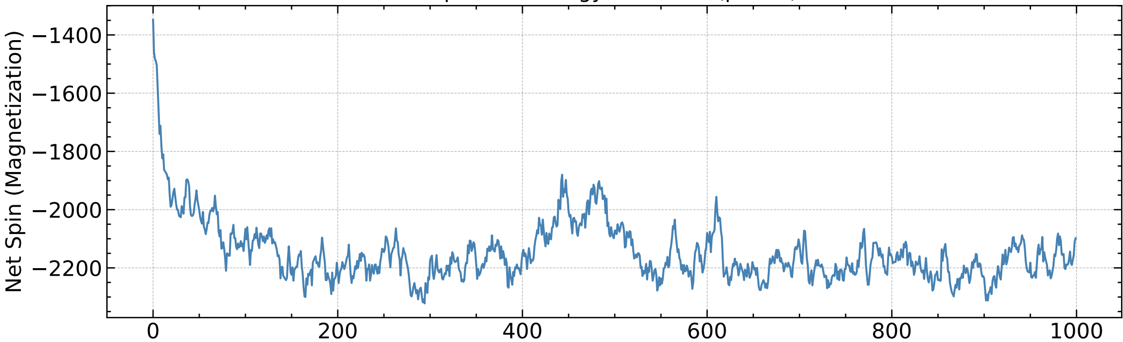
Spin and Energy Evolution ( \beta=0.5 )
