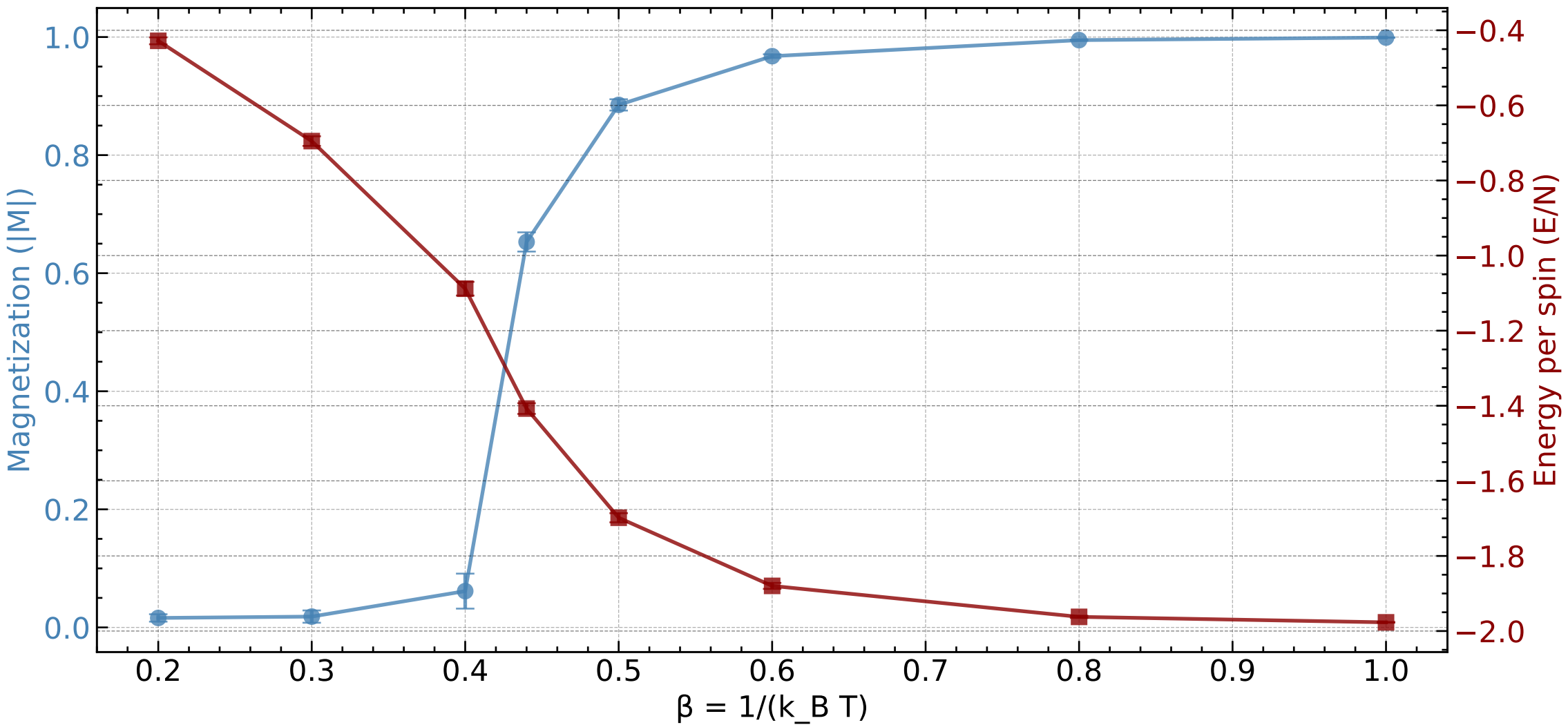
Phase Diagram: Magnetization and Energy vs Temperature
