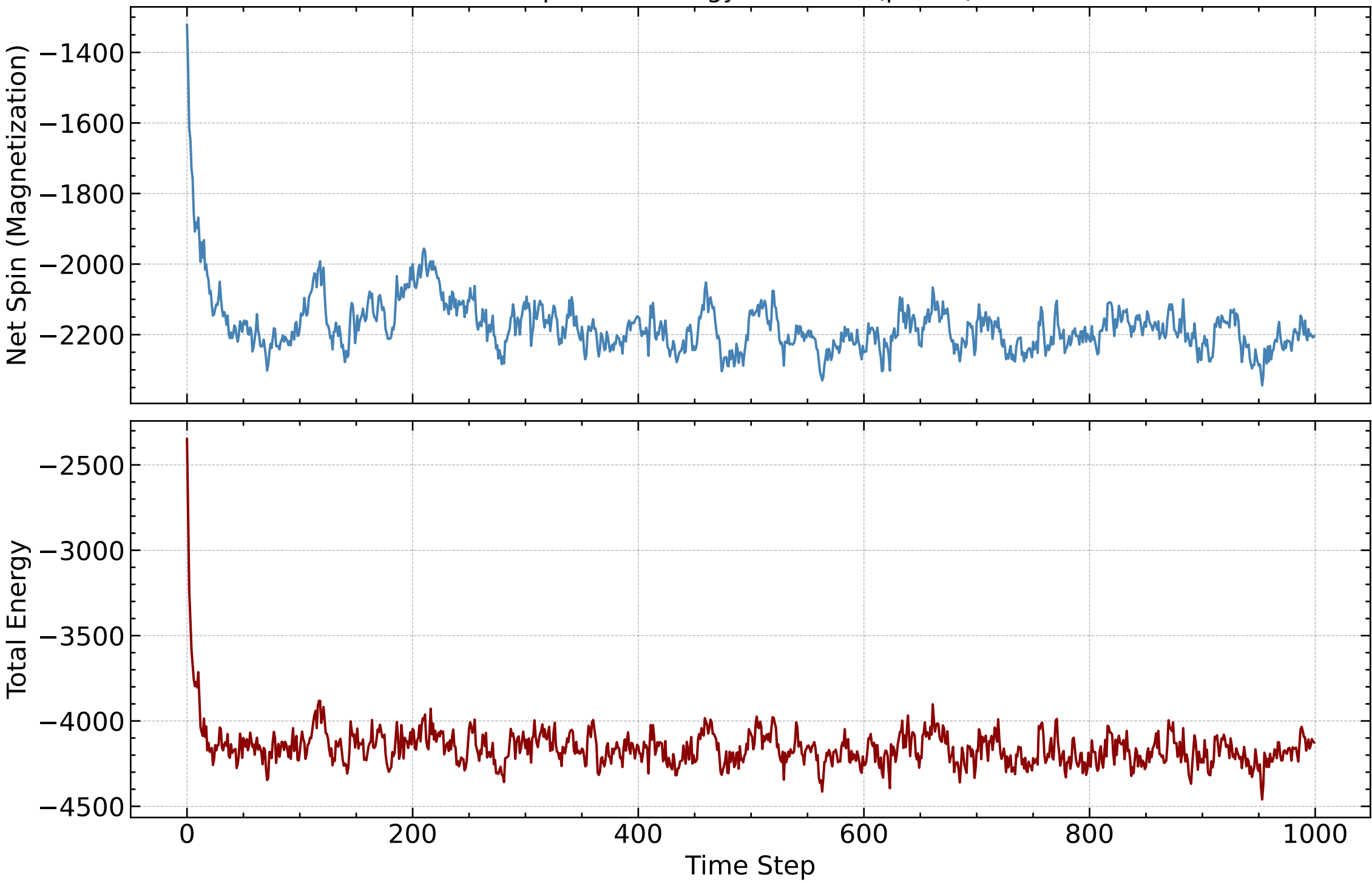
Spin and Energy Evolution ( \beta=0.5 )
