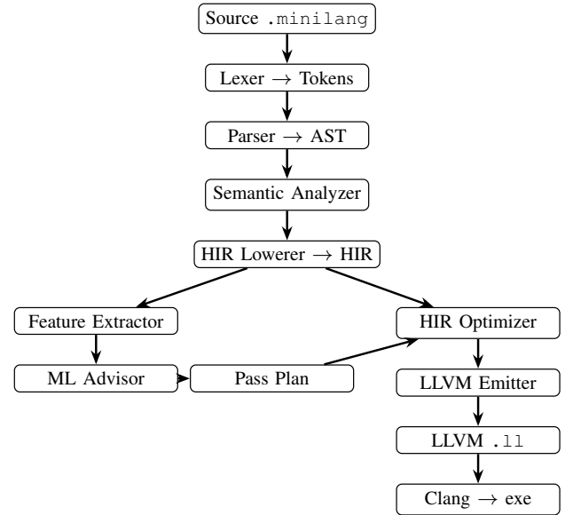
Fig. 1: Data flow.
