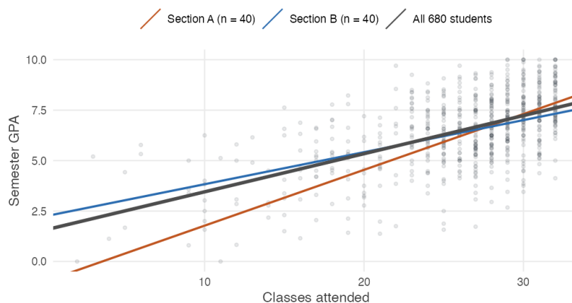
Figure 6.2: Two sections of forty students, each with its own fitted line, against the line fitted to all 680. Neither section's line is the population regression function, and from a single section there would be no way to tell how far off it was.
