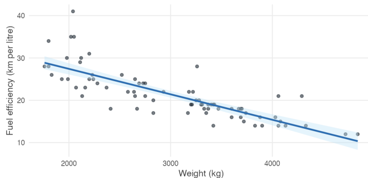
Figure 6.4: Fuel efficiency against weight for 74 cars, with the fitted line.
