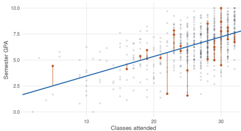
Figure 6.3: The fitted line, with the vertical distances it misses by shown for a handful of students. Ordinary least squares chooses the line making the sum of those squared distances as small as possible.
