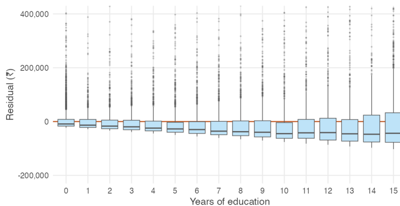
Figure 7.3: Residuals from a regression of annual earnings on years of schooling, shown as a boxplot at each level of education. The boxes widen steadily to the right: errors are far more variable where schooling is high. Homoskedasticity would appear as boxes of constant height. A few extreme residuals lie above the range plotted.
