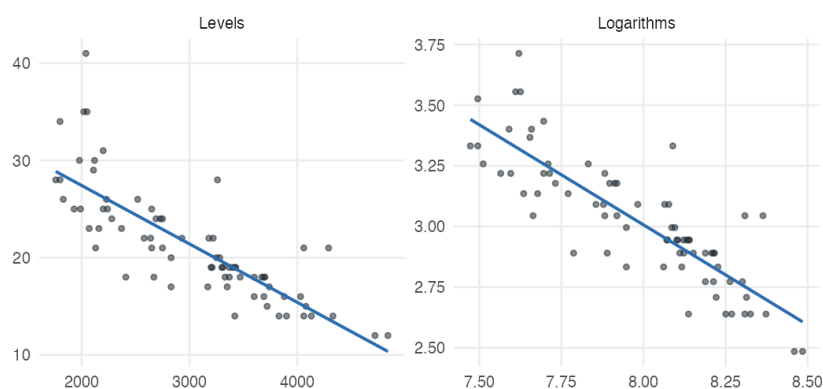
Figure 7.4: The same 74 cars in levels and in logarithms. Both look broadly linear; the logarithmic version is a little tighter around the line, which is the improvement in R-squared from 0.65 to 0.71. The gain here is real but modest – the case for the log form rests mainly on interpretation.
