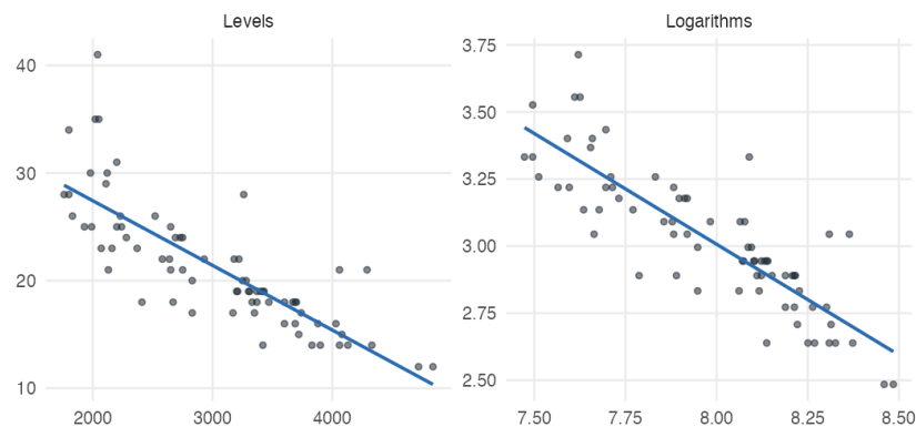
Figure 7.8: The same 74 cars in levels and in logarithms. Both look broadly linear; the logarithmic version is a little tighter around the line, which is the improvement in R -squared from 0.65 to 0.71 . The gain here is real but modest – the case for the log form rests mainly on interpretation.
