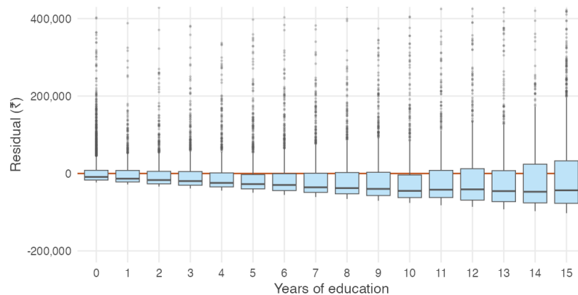
Figure 7.6: Residuals from a regression of annual earnings on years of schooling, shown as a boxplot at each level of education. The boxes widen steadily to the right: errors are far more variable where schooling is high. Homoskedasticity would appear as boxes of constant height. A few extreme residuals lie above the range plotted.
