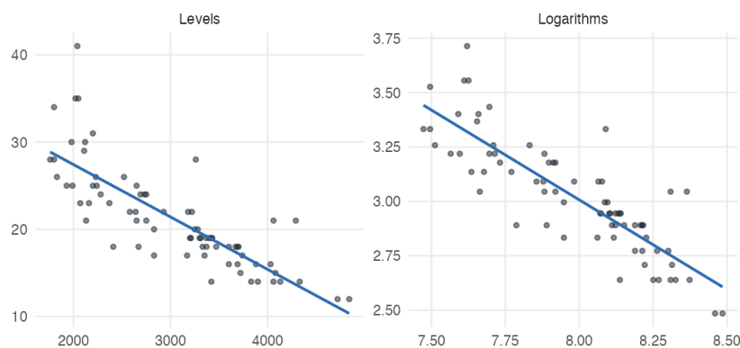
Figure 7.7: The same 74 cars in levels and in logarithms. Both look broadly linear; the logarithmic version is a little tighter around the line, which is the improvement in R -squared from 0.65 to 0.71 . The gain here is real but modest—the case for the log form rests mainly on interpretation.
