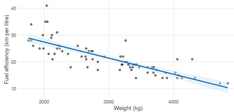
Figure 7.8: Fuel efficiency against weight for 74 cars, with the fitted line.
