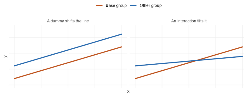
Figure 10.1: The two things a group variable can do. On the left the groups differ only in level, which is all a dummy on its own can express. On the right they differ in level and in rate of change, which requires an interaction term.
