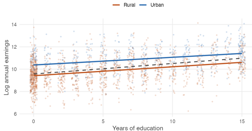
Figure 10.2: Log earnings against education for rural and urban workers, with a 2,000-worker sample drawn for legibility. The solid lines are fitted separately to each group; the dashed line is the single pooled regression that ignores residence. The two group lines differ in level and, less obviously, in steepness – the urban line is slightly flatter. The pooled line describes neither group.
