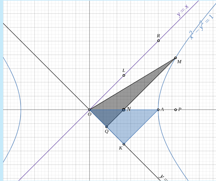
Figure 40: Triangles Have the Same Area
