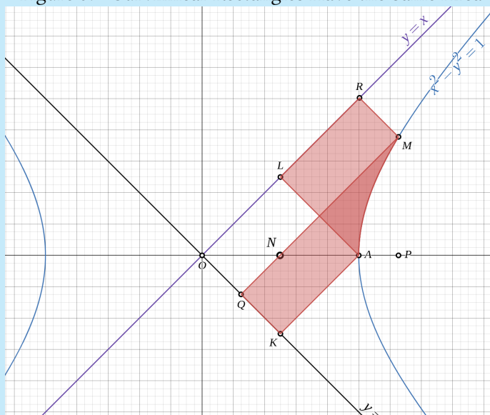
Figure 39: Curvilinear Rectangles Have the Same Area
