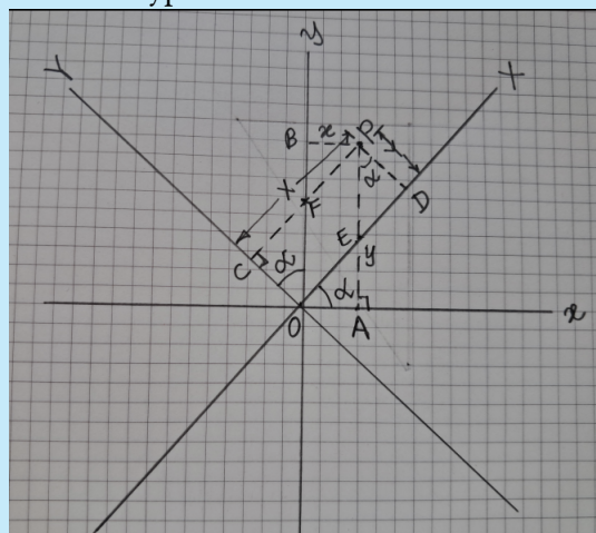
Figure 13: The Hyperbola in a Rotated Coordinate System
