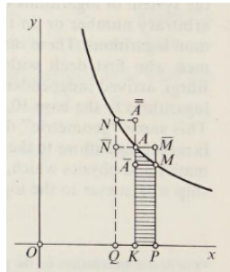
Figure 34: Estimating the value of e with \ln(1 + \frac{1}{n})
