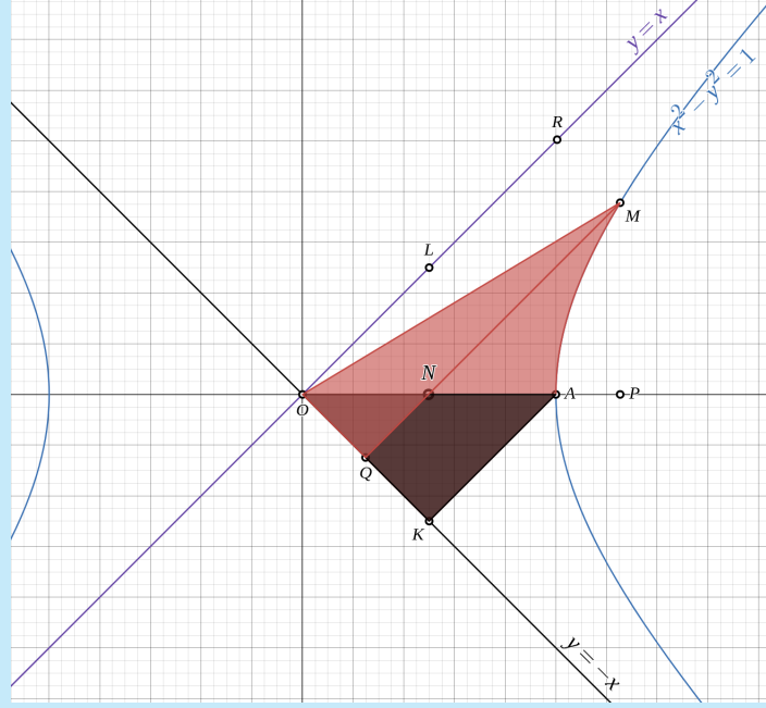
Figure 41: Areas of QKAM , RLAM , and OAM are the Same
