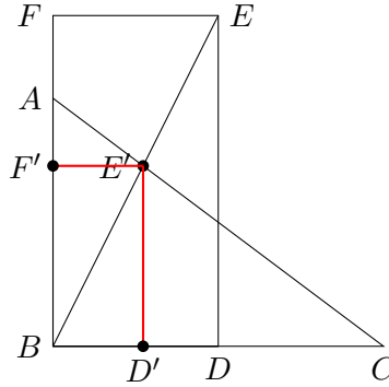
Figure 6: The Scaled rectangle.
