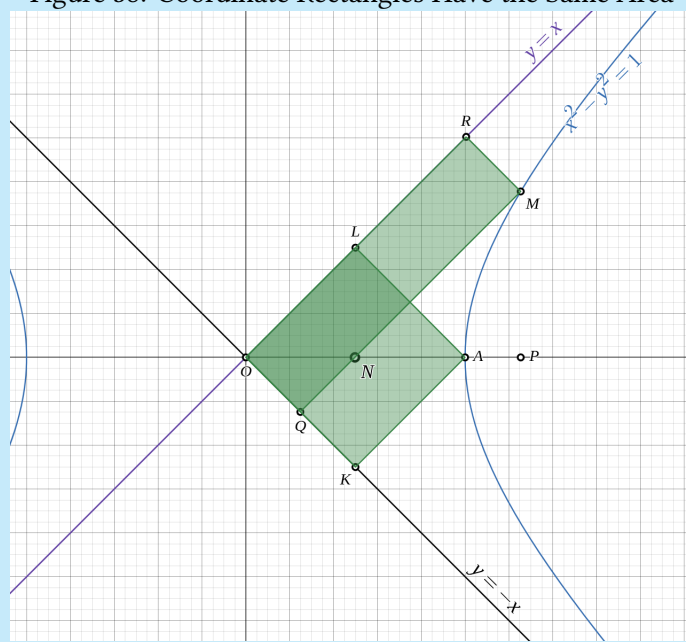
Figure 38: Coordinate Rectangles Have the Same Area
