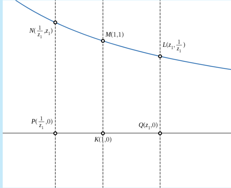
Figure 36: S(z_1) + S(\frac{1}{z_1}) for z_1 > 1
