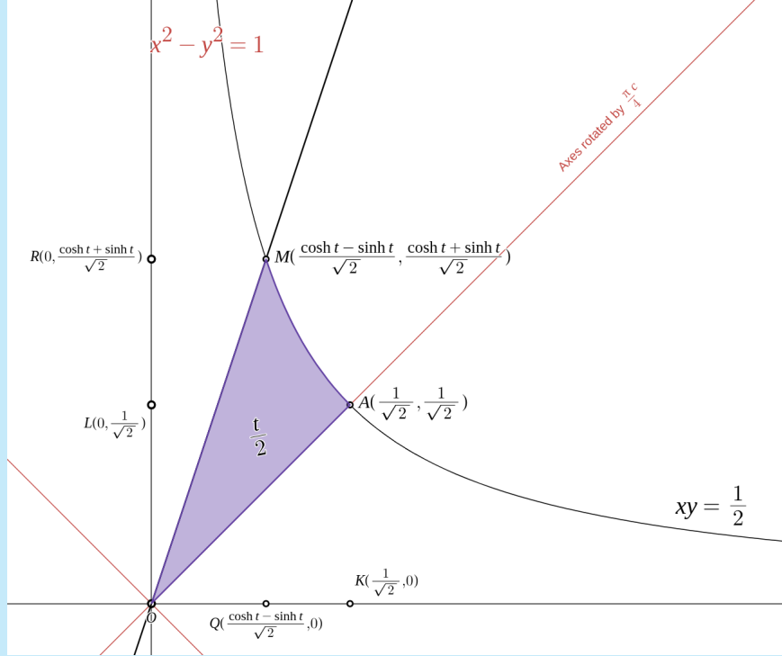
Figure 37: Certain Coordinates Concerning the Hyperbola xy = \frac{1}{2} in the Two Systems
