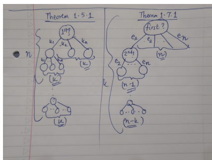
Figure 1.2: Comparing the Number of n -strings of k Elements with that of Ordered k -subsets of an n -set
