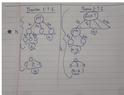
Figure 1.2: Comparing the Number of n -strings of k Elements with that of Ordered k -subsets of an n -set
