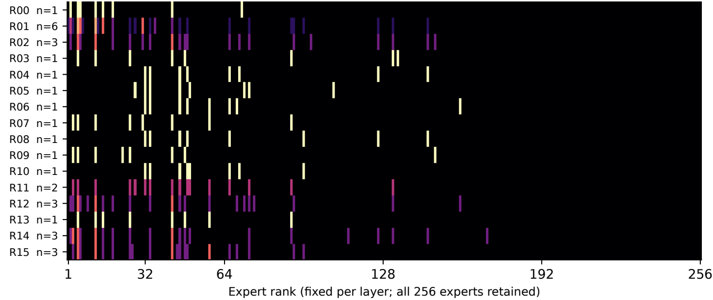
Layer 10 | Accepted this step | tokens=30, requests=16/16
