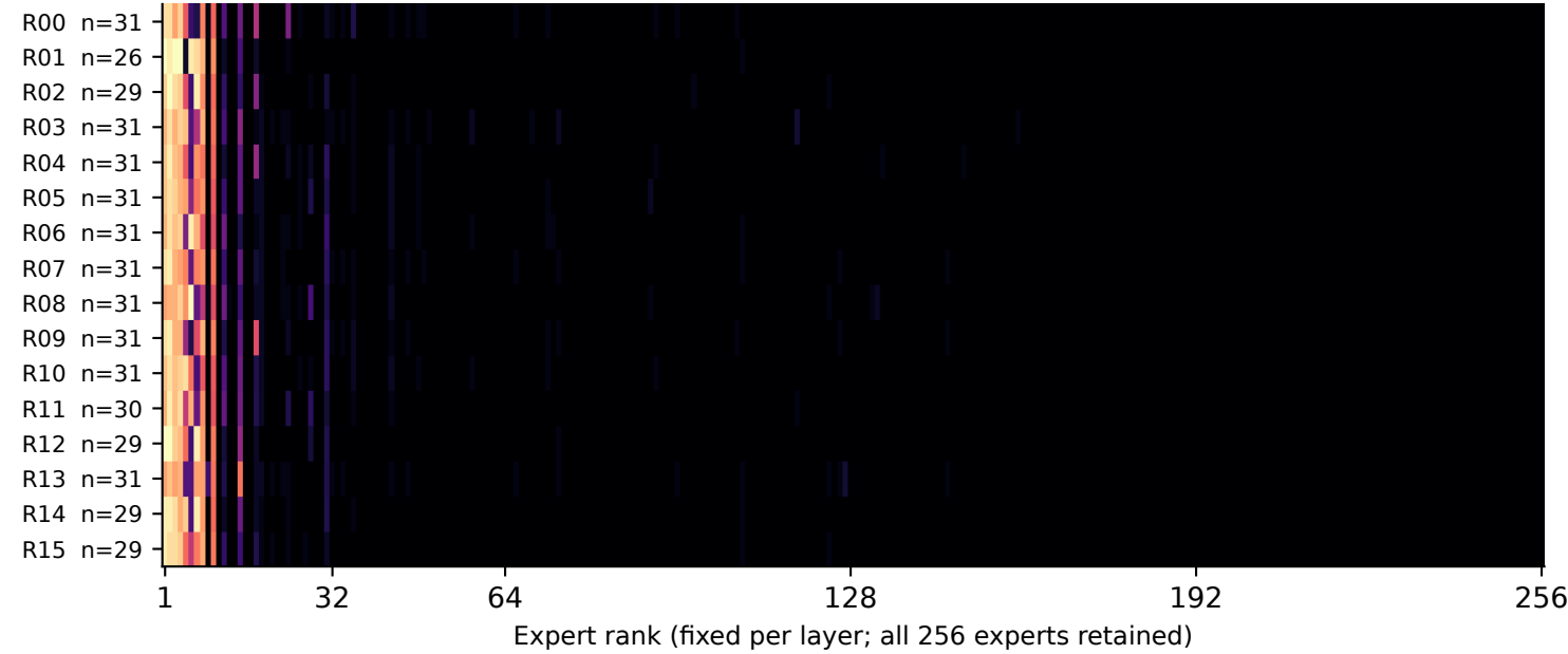
Layer 10 | Unresolved this step | tokens=482, requests=16/16
