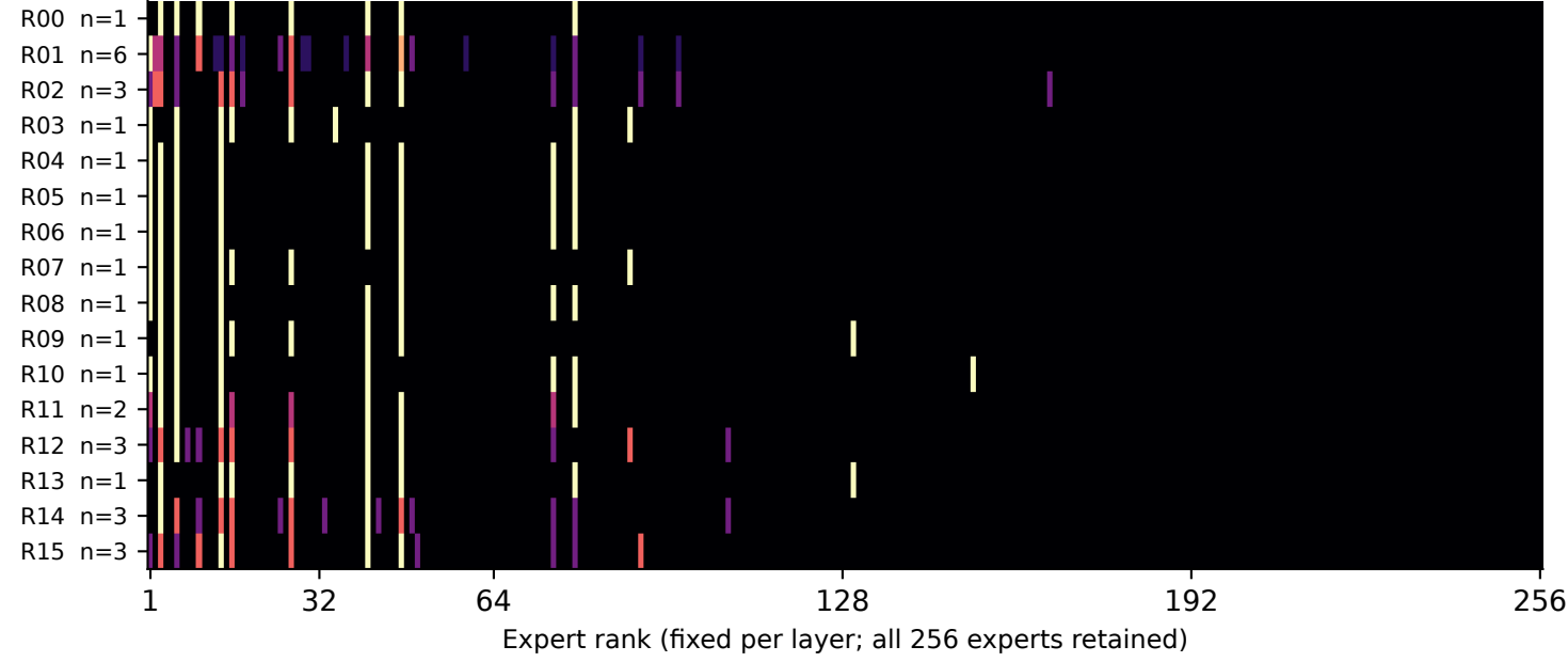
Layer 18 | Accepted this step | tokens=30, requests=16/16
