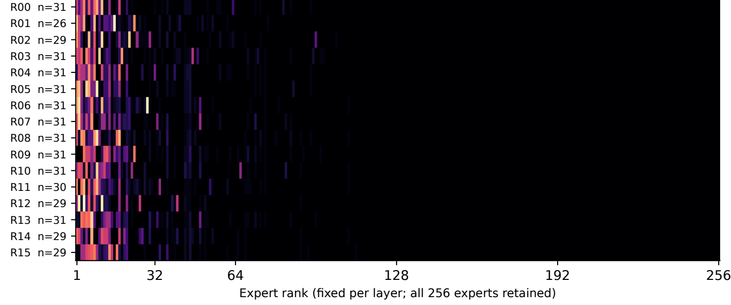
Layer 18 | Unresolved this step | tokens=482, requests=16/16
