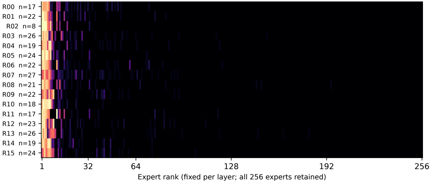
Layer 10 | Unresolved this step | tokens=335, requests=16/16
