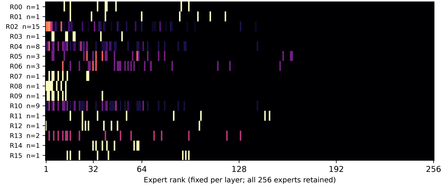
Layer 10 | Accepted this step | tokens=50, requests=16/16
