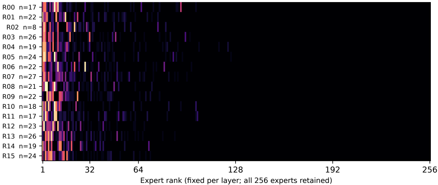
Layer 18 | Unresolved this step | tokens=335, requests=16/16
