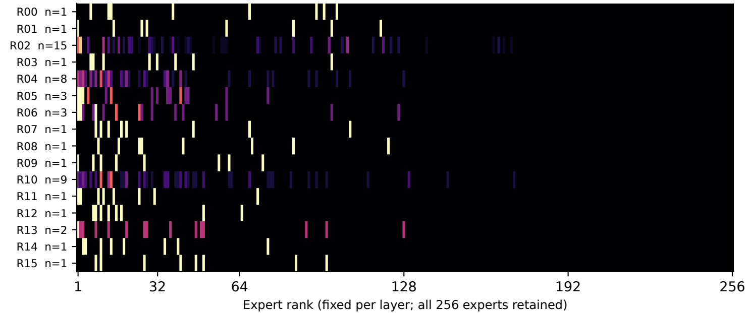
Layer 18 | Accepted this step | tokens=50, requests=16/16
