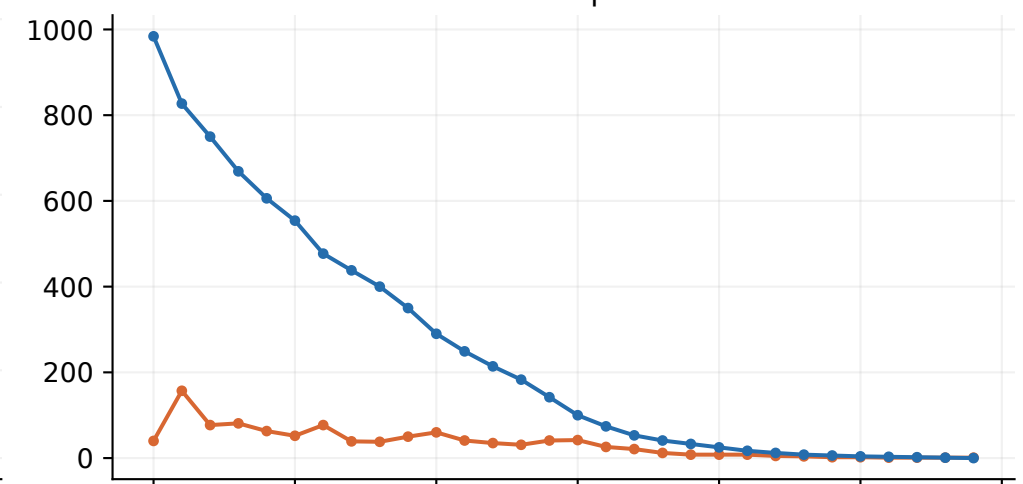
HumanEval | batch 8
