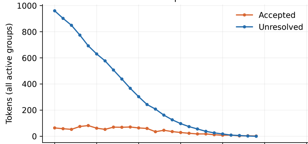
GSM8K | batch 8
