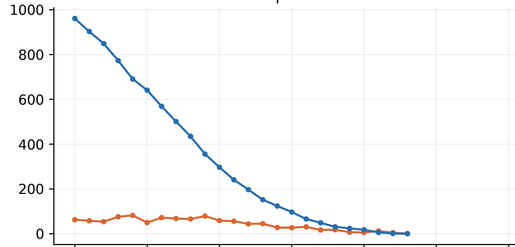
GSM8K | batch 16
