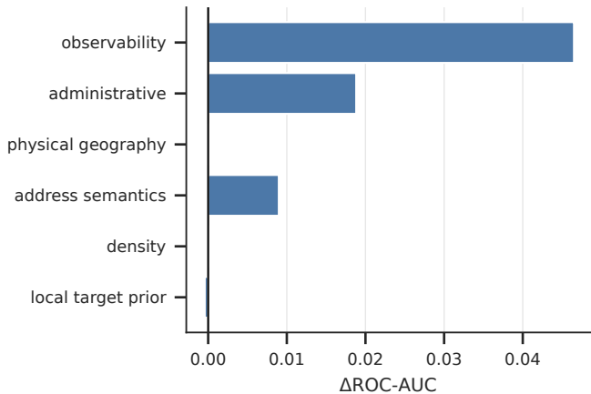
a Address blocks, Global
