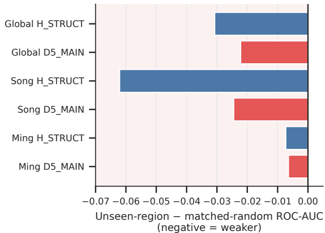
b Unseen-region transport
