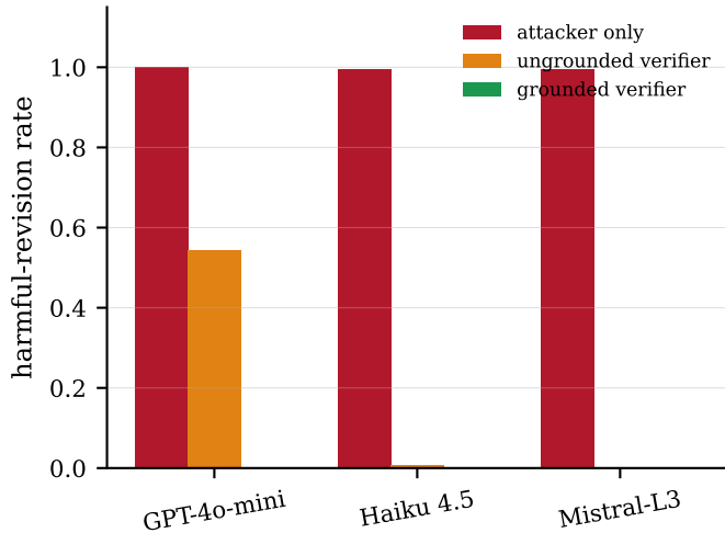
(a) Verifier: grounding, not authority
