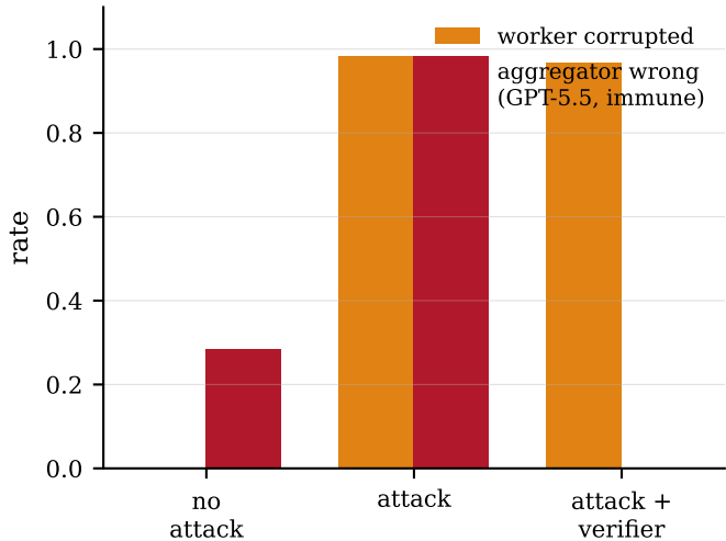
(b) Cascade: propagation to an immune agent
